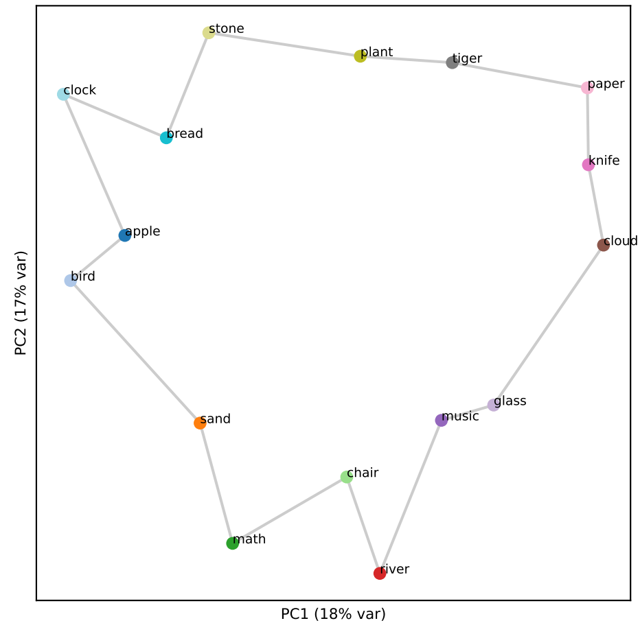
Qwen L33 (RSA 0.88)
