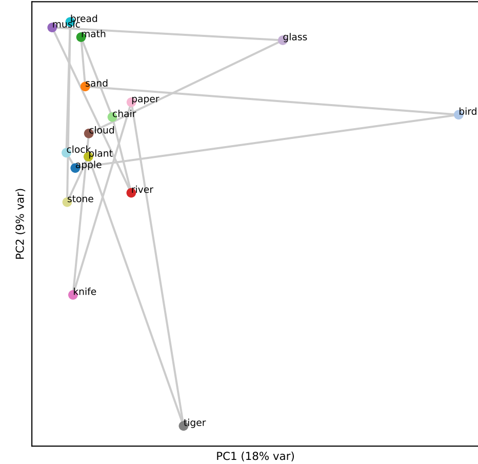
Qwen L6 (RSA -0.02)
