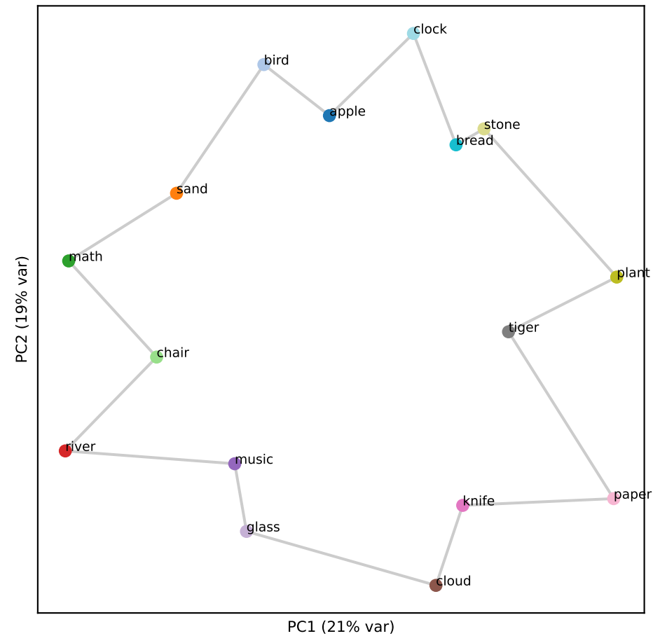
Qwen L34 (RSA 0.87)
