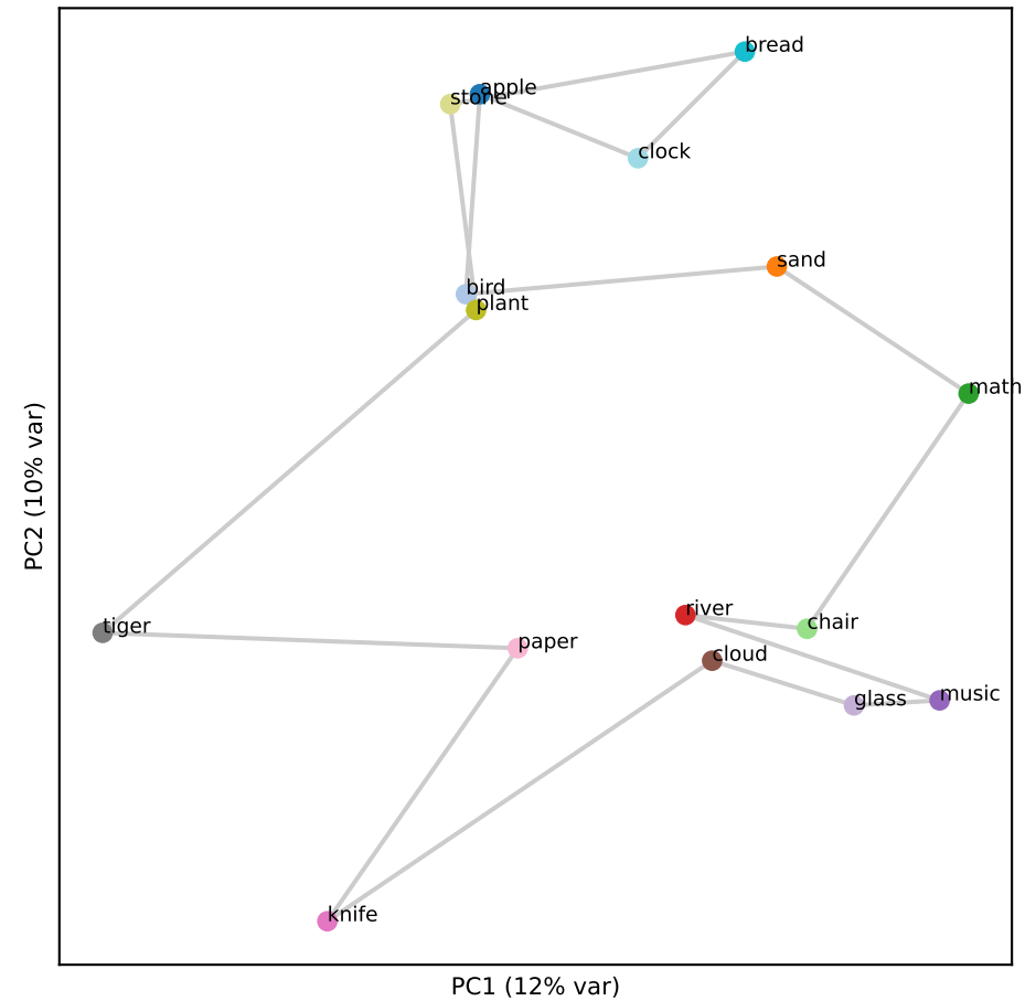
Qwen L21 (RSA 0.55)
