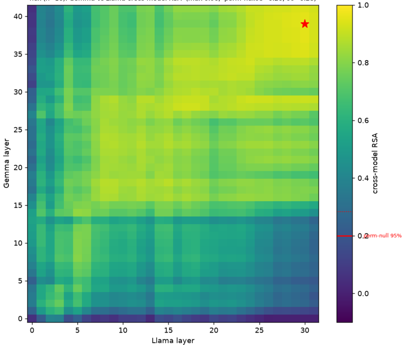
hex (n=16): Gemma vs Llama cross-model RSA (max 0.96; perm-null95=0.20, 99=0.28)
