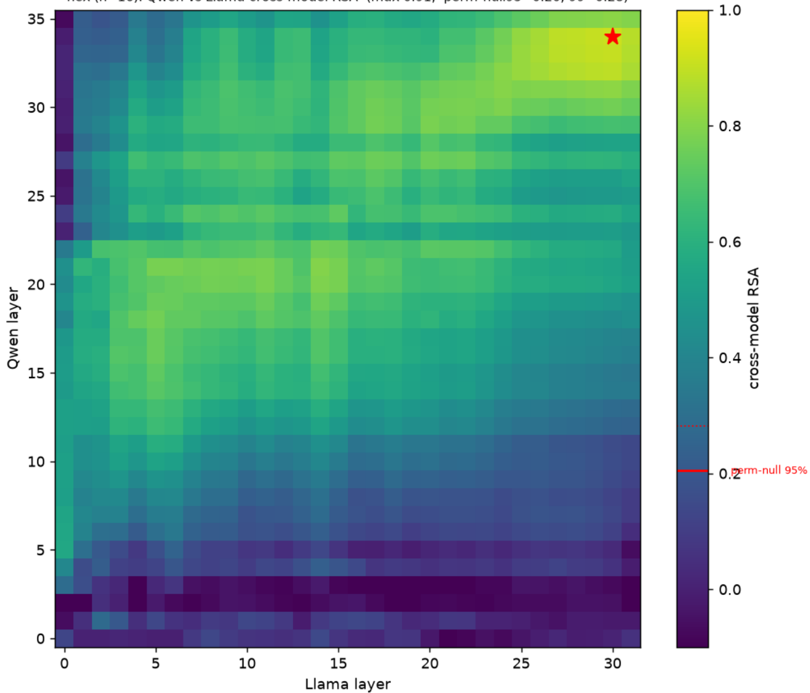
hex (n=16): Qwen vs Llama cross-model RSA (max 0.91; perm-null95=0.20, 99=0.28)
