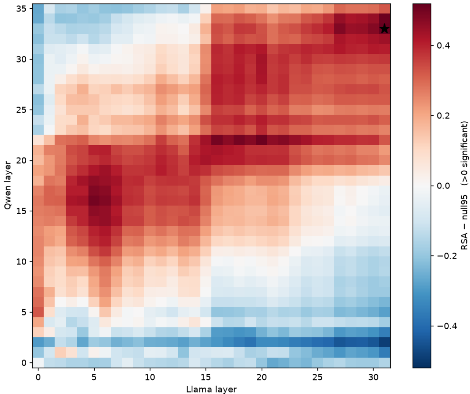
square_grid (n=16): Qwen vs Llama RSA – perm-null95 (0.18) red = above chance (significant); 68% of cells significant
