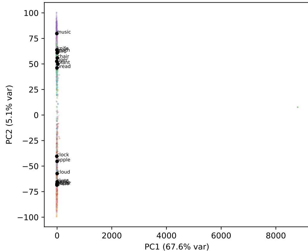
Qwen L28
