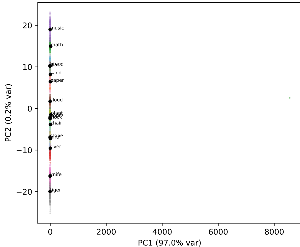
Qwen L14
