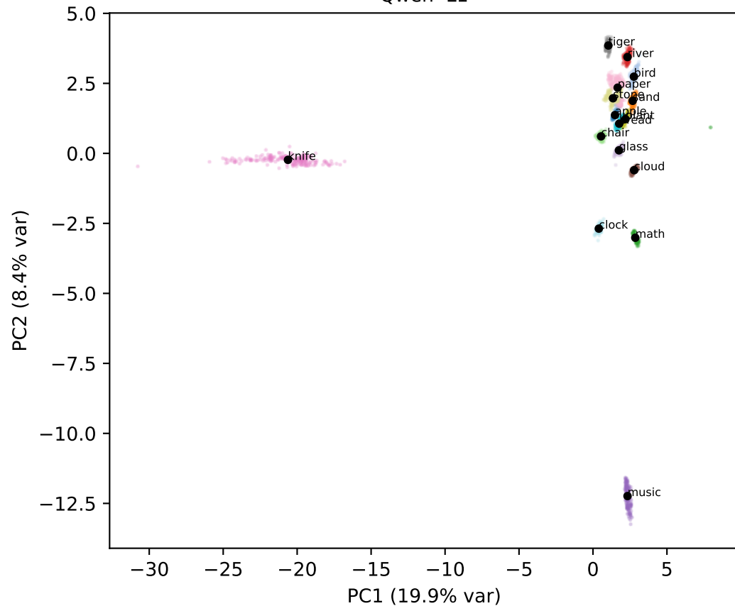
Qwen L1
