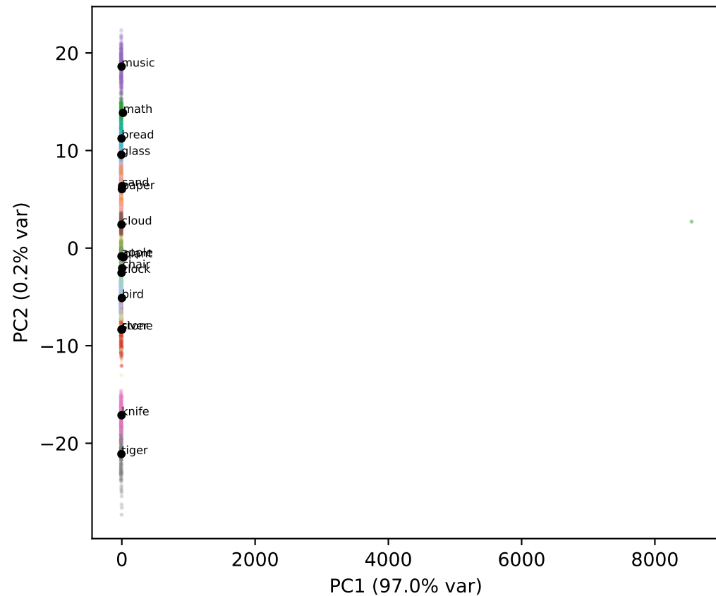
Qwen L15
