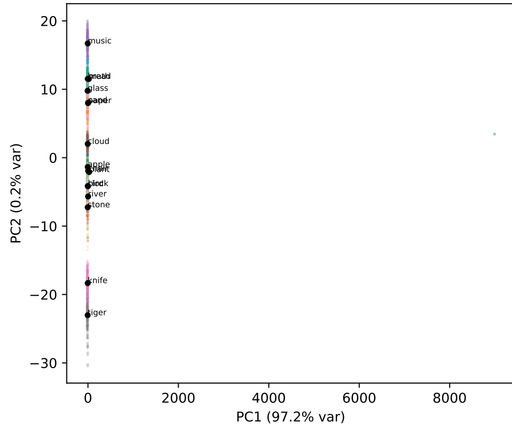
Qwen L16
