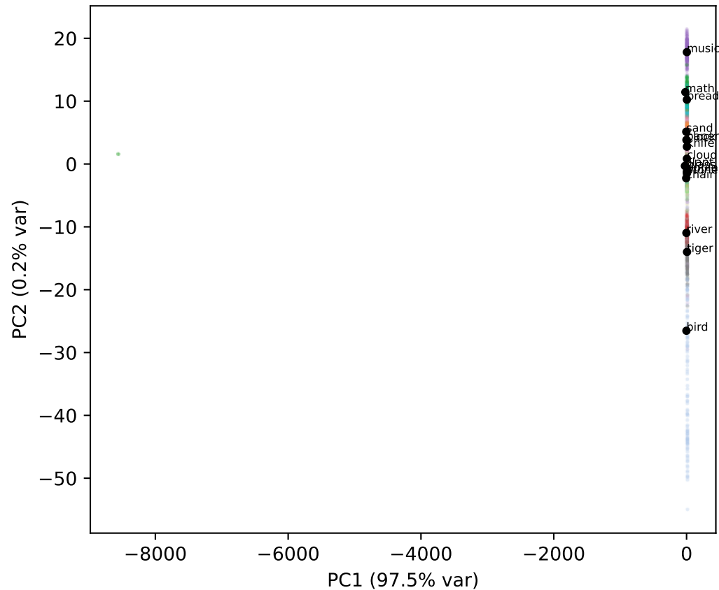
Qwen L8
