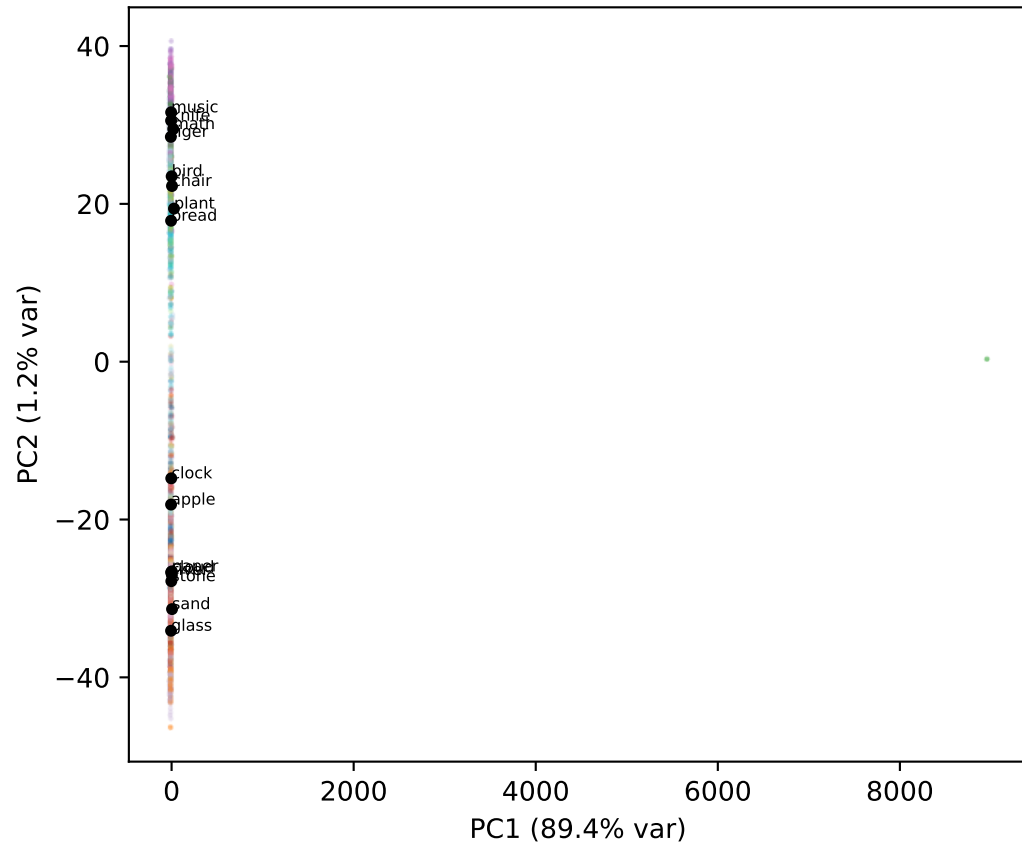
Qwen L22
