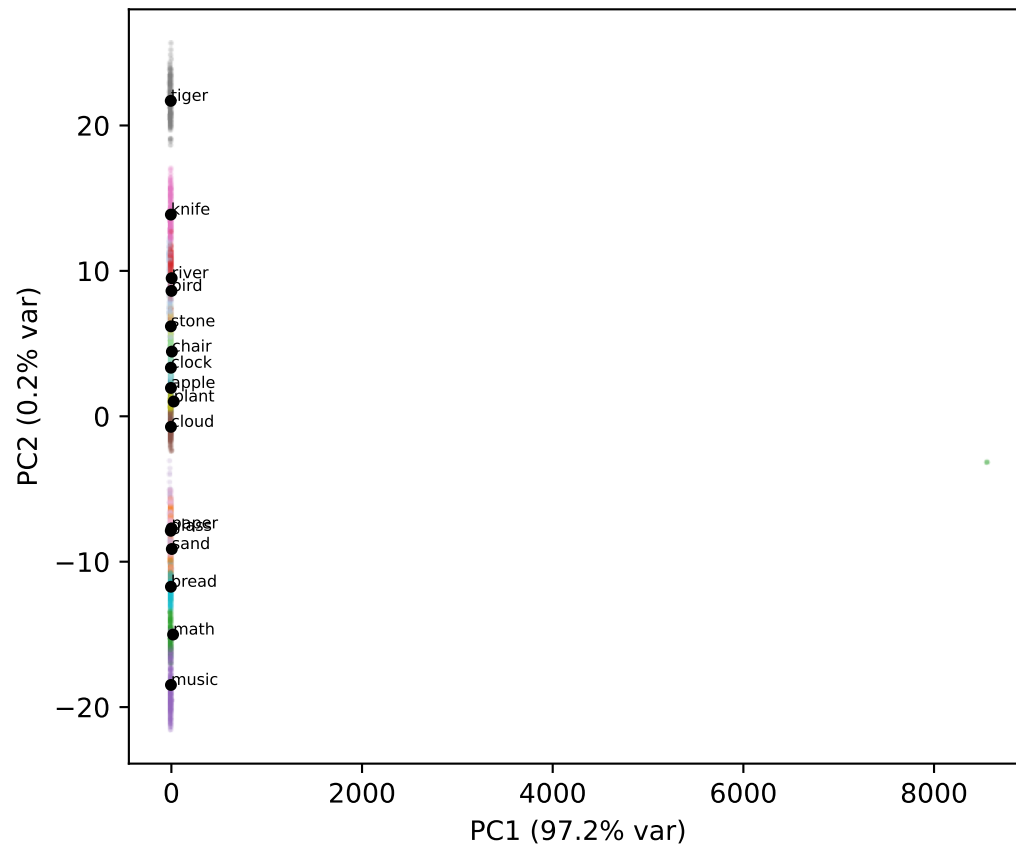
Qwen L12
