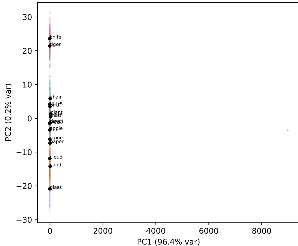
Qwen L18
