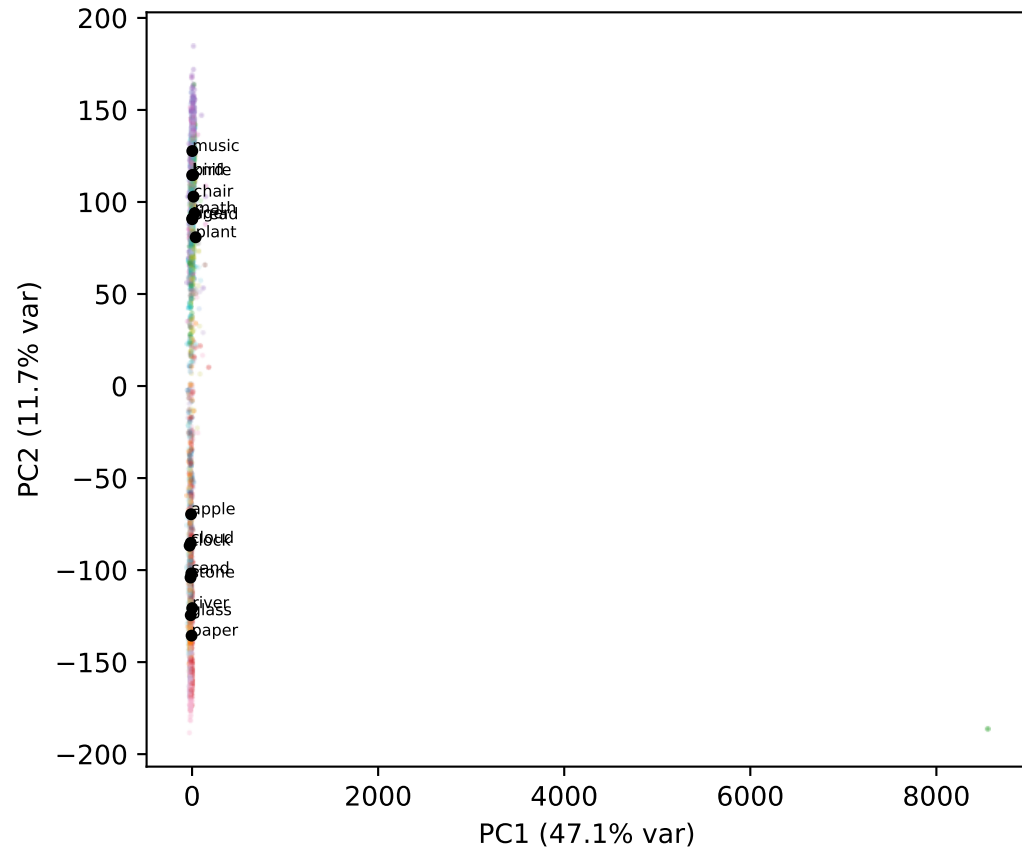
Qwen L32
