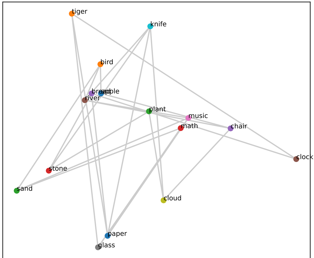
Gemma L0 (grid RSA=-0.00, PCA corr=-0.11)
