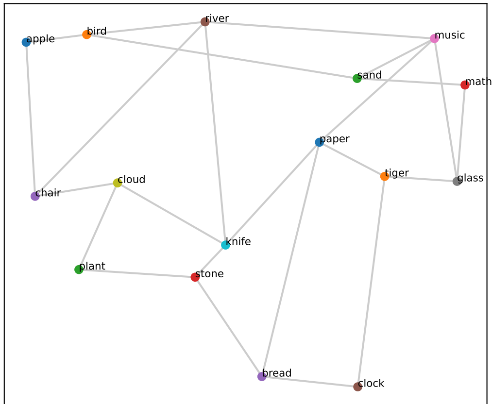
Gemma L21 (grid RSA=0.60, PCA corr=0.73)
