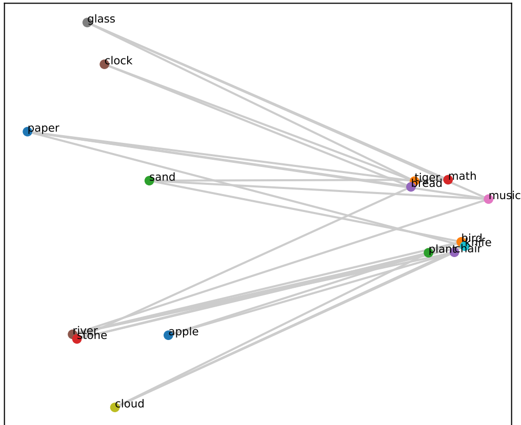
Qwen L34 (grid RSA=0.18, PCA corr=-0.00)
