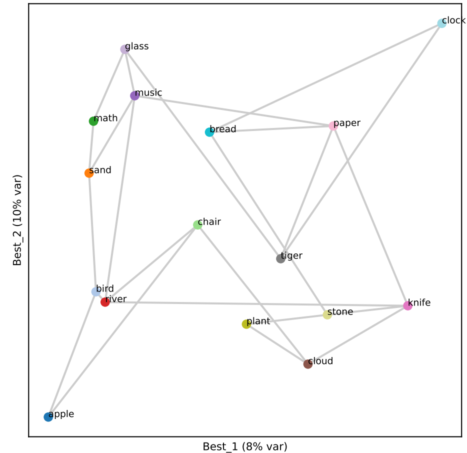
Qwen L26 (RSA 0.42)
