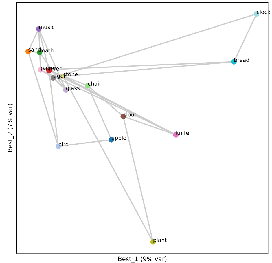
Qwen L2 (RSA 0.26)
