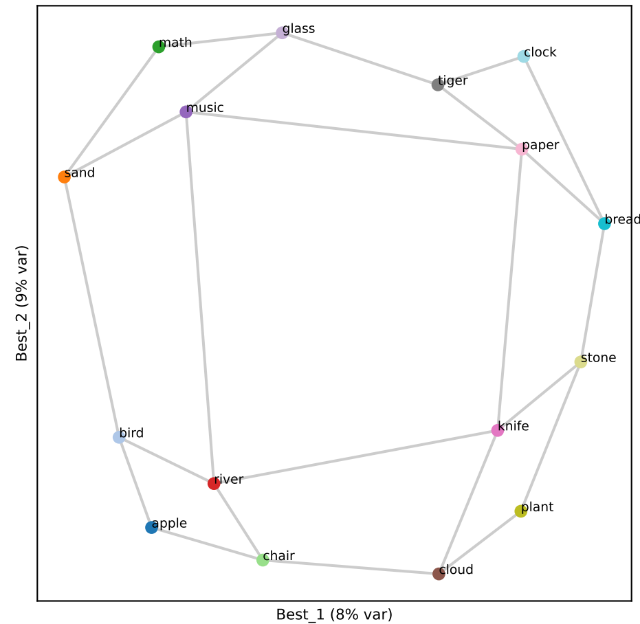
Qwen L35 (RSA 0.84)
