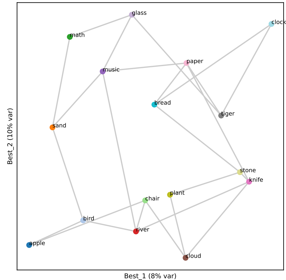
Qwen L27 (RSA 0.59)
