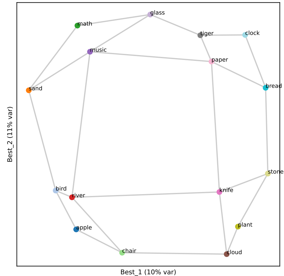
Qwen L34 (RSA 0.84)
