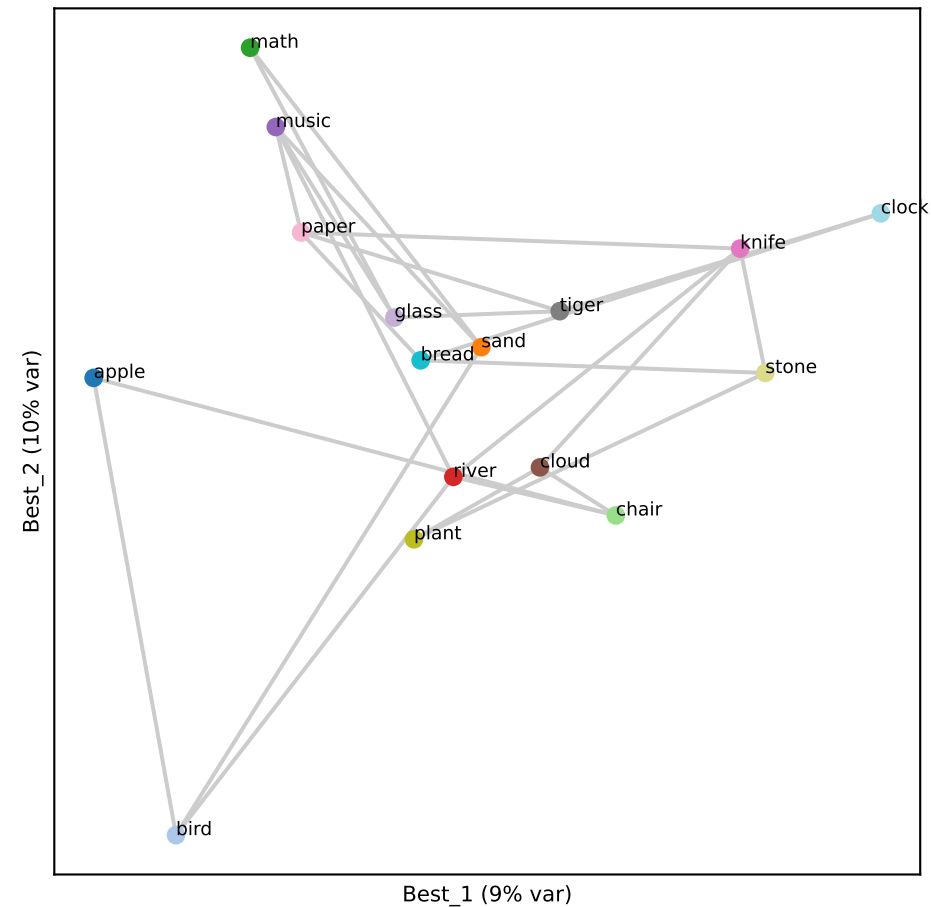
Qwen L14 (RSA 0.15)
