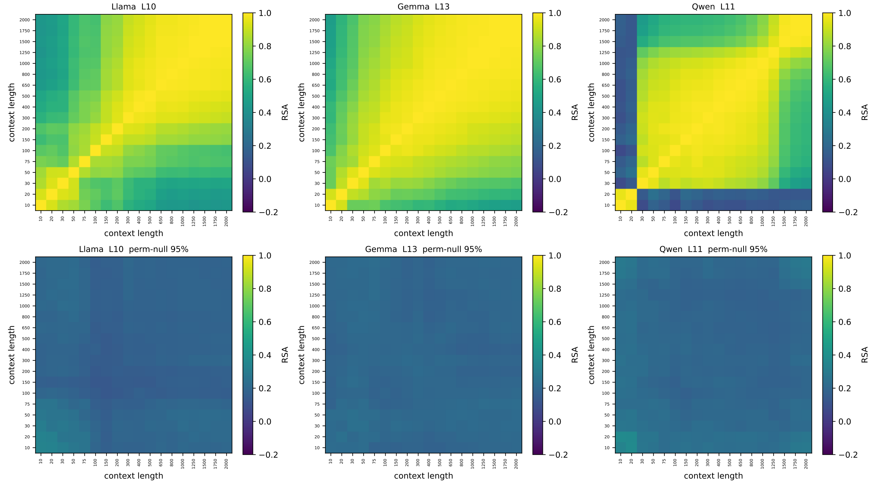
square_grid [v2] context-vs-context node-geometry RSA — relative depth 0.32 top: observed | bottom: node-label permutation null (95th pct)
