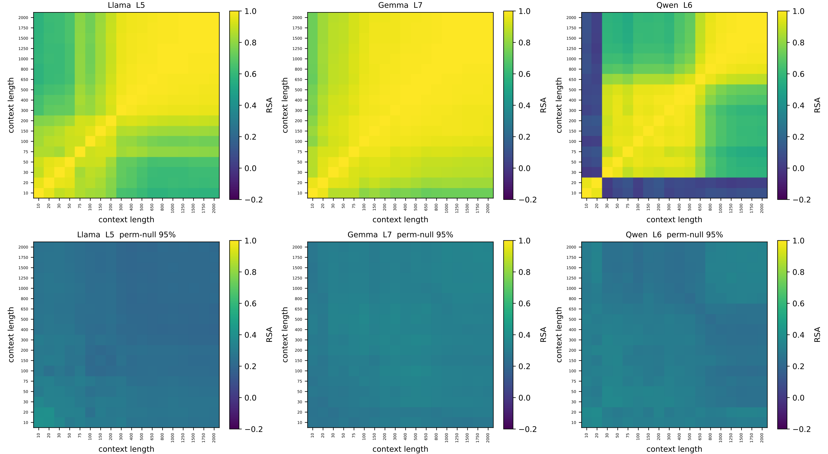
square_grid [v2] context-vs-context node-geometry RSA — relative depth 0.17 top: observed | bottom: node-label permutation null (95th pct)
