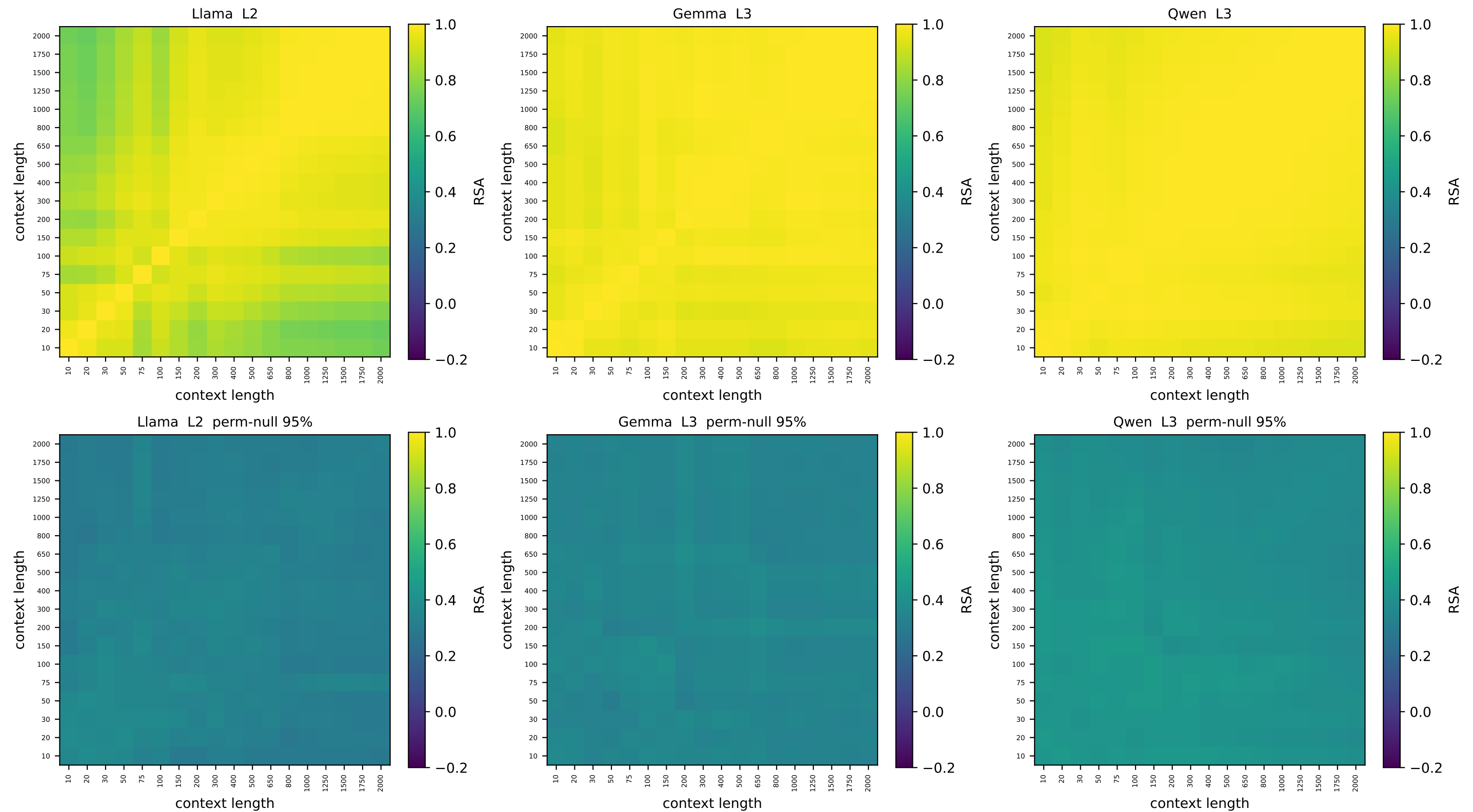
square_grid [v2] context-vs-context node-geometry RSA — relative depth 0.07 top: observed | bottom: node-label permutation null (95th pct)
