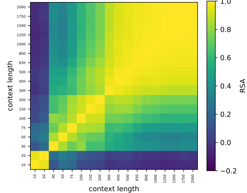
Qwen L24 perm-null 95%
