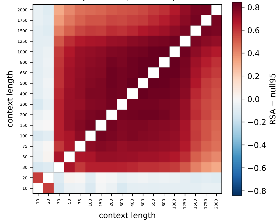
Qwen L14 (81% > null)
