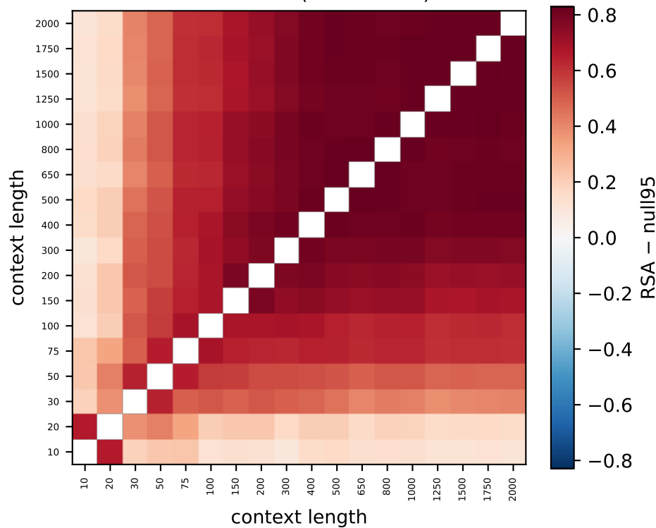
Gemma L18 (100% > null)
