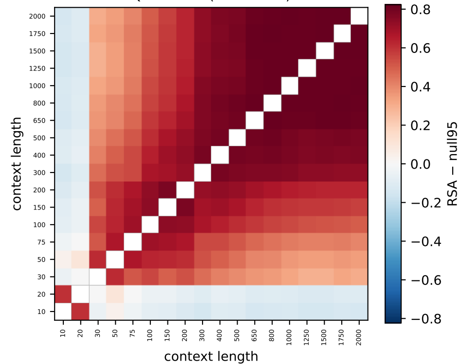
Qwen L22 (80% > null)
