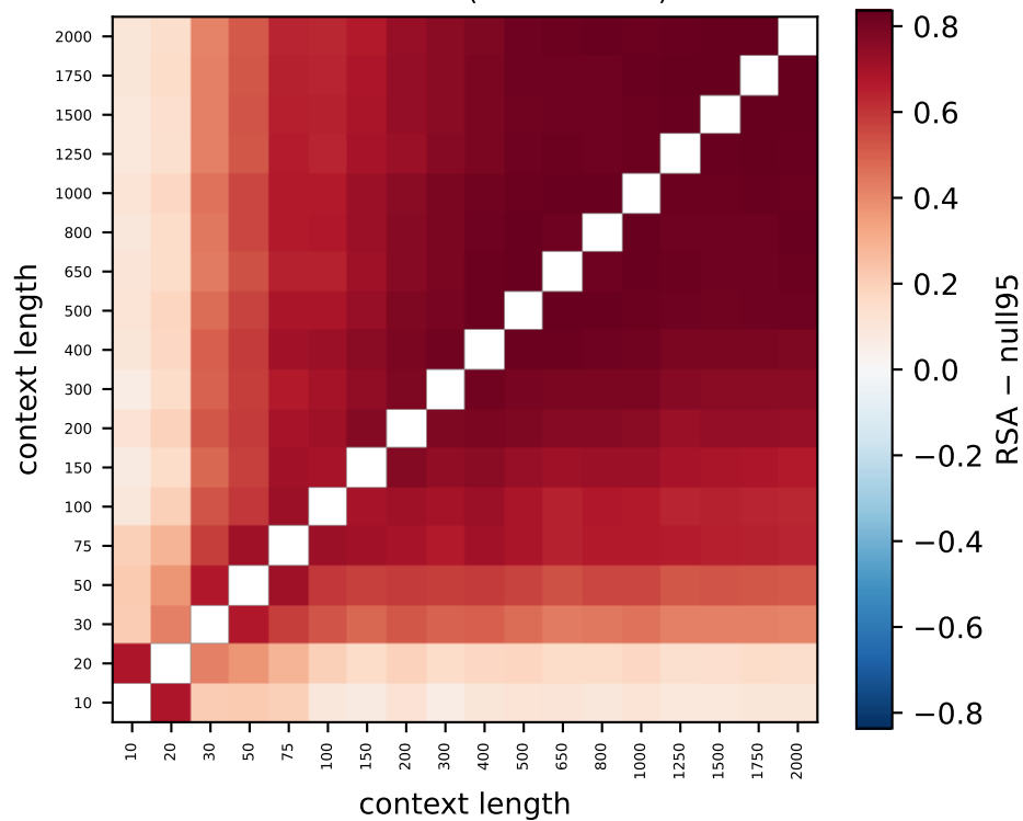
Gemma L19 (100% > null)
