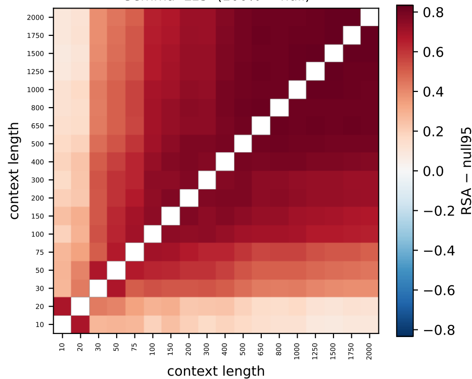
Gemma L15 (100% > null)
