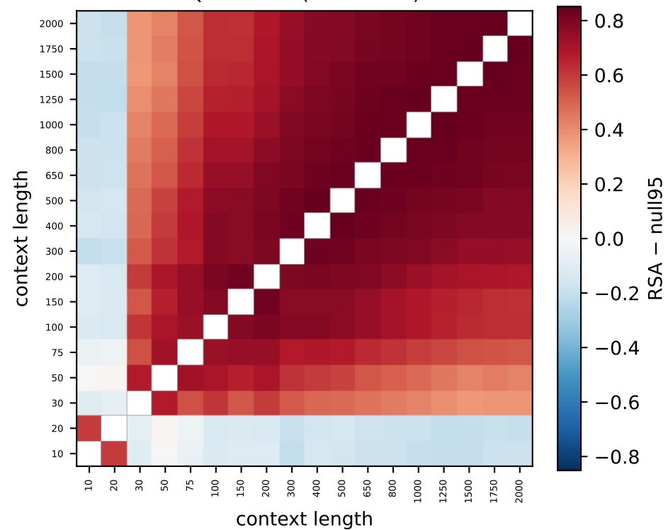
Qwen L20 (80% > null)
