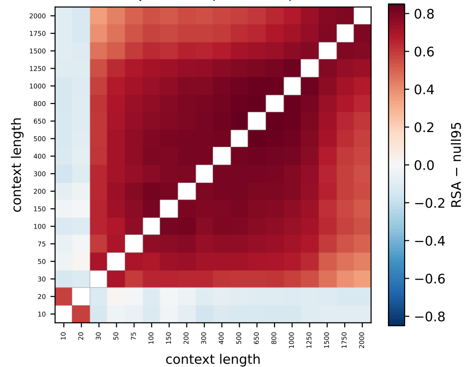
Qwen L15 (80% > null)
