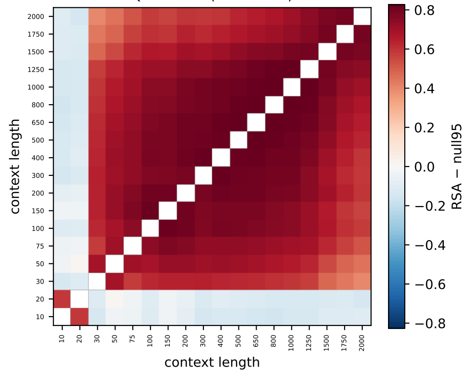
Qwen L16 (80% > null)
