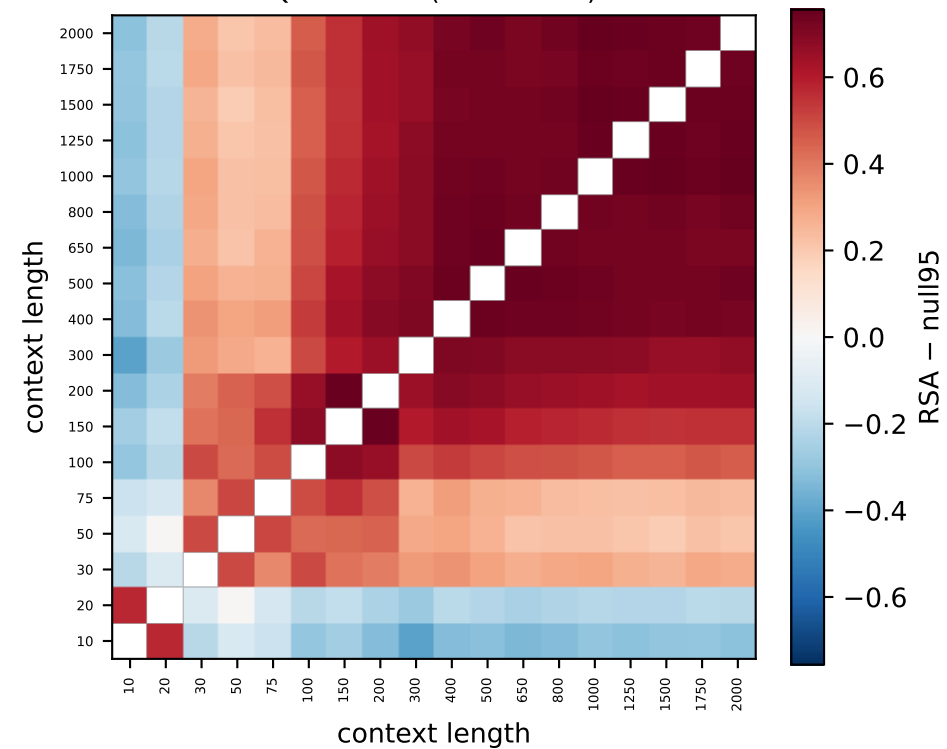
Qwen L25 (80% > null)
