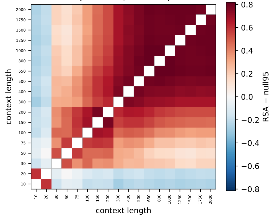
Qwen L24 (80% > null)
