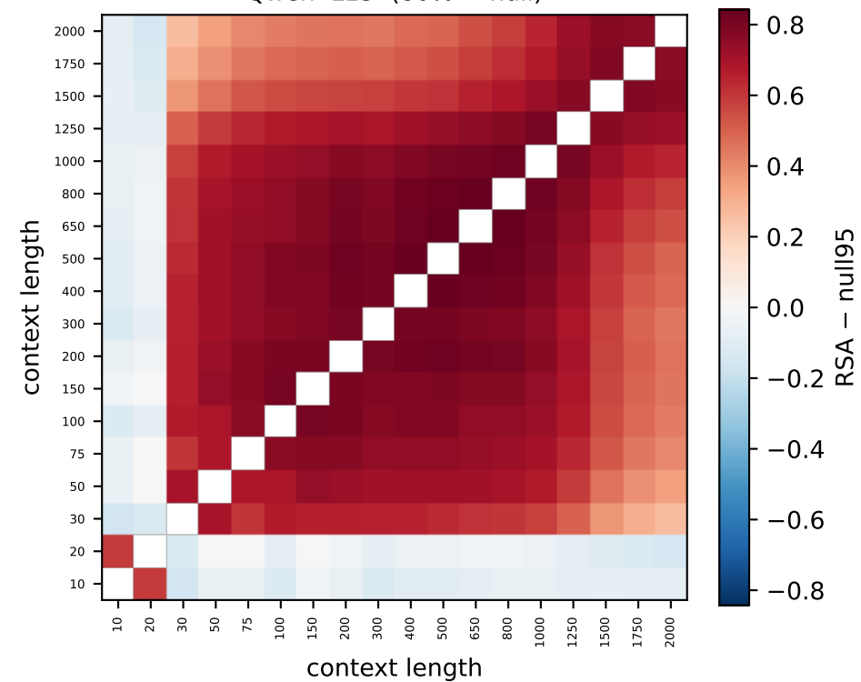
Qwen L13 (80% > null)
