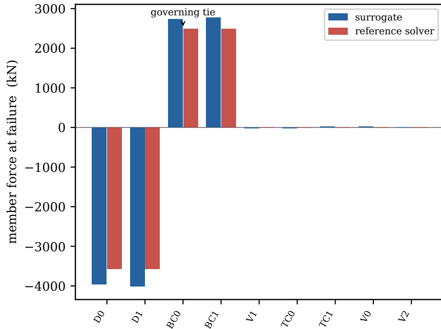
(b) force state at the optimum
