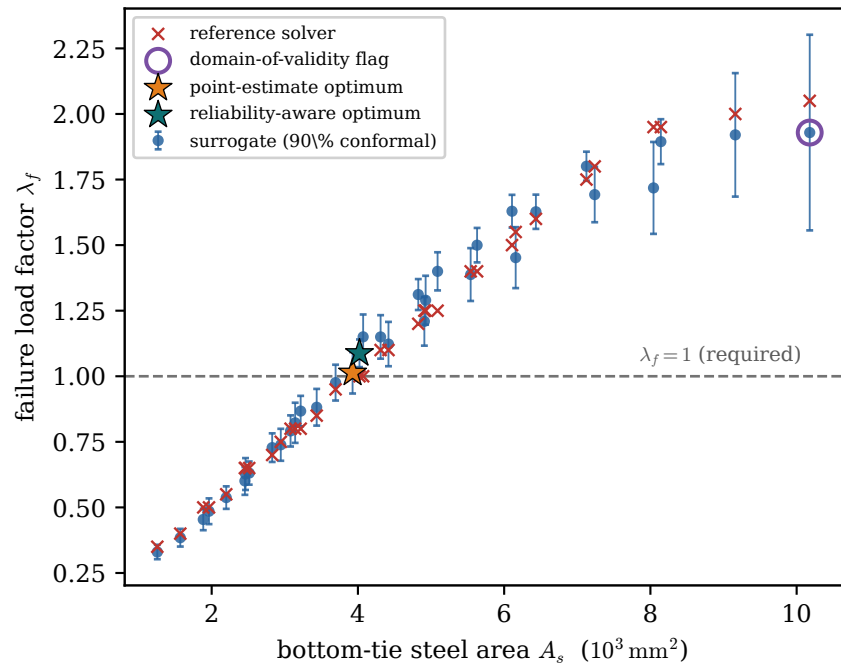
(a) reinforcement minimisation
