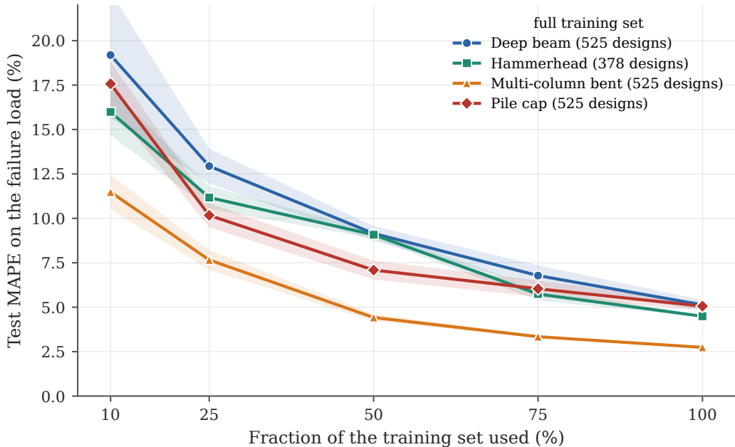
(a) Learning curves: mean of three subsamples, band one standard deviation
