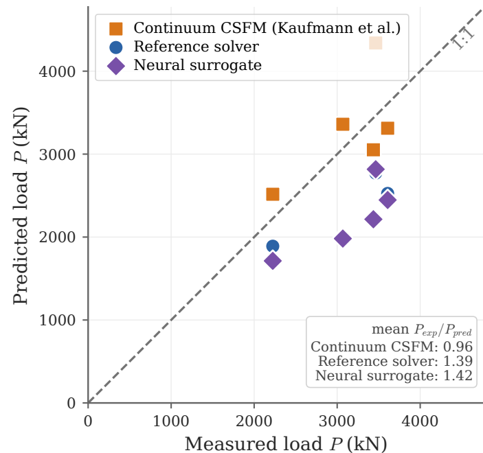
(a) Predicted against measured load
