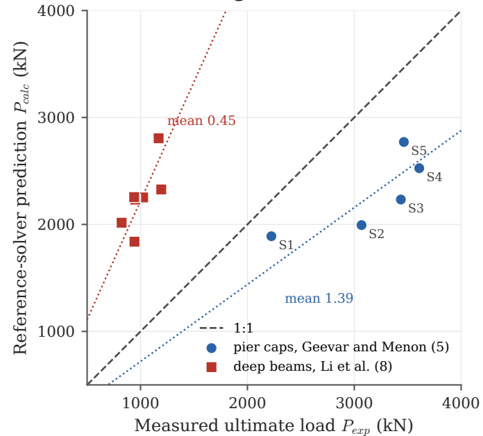
(a) Predicted against measured load
