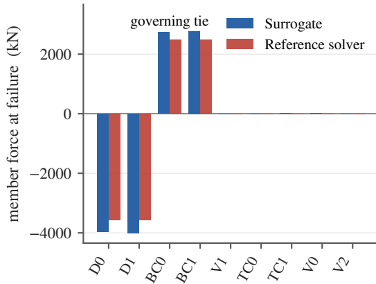
(b) Force state at the optimum
