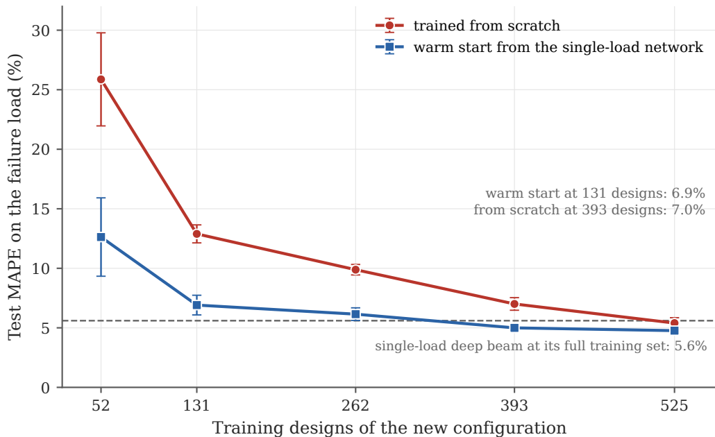
(a) Two-point-load deep beam: accuracy against training designs
