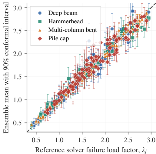
(a) Ensemble mean and 90% interval
