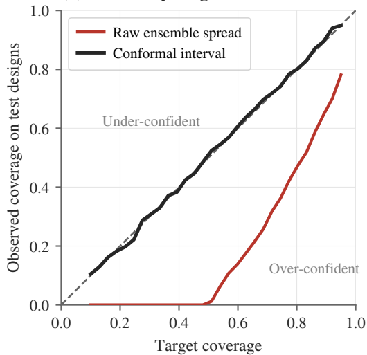
(b) Reliability diagram
