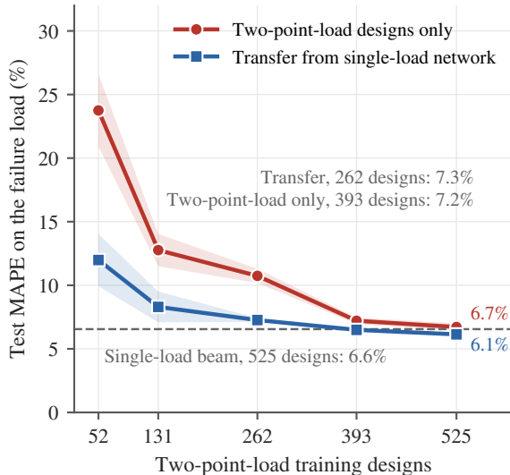
(b) Test error against training designs
