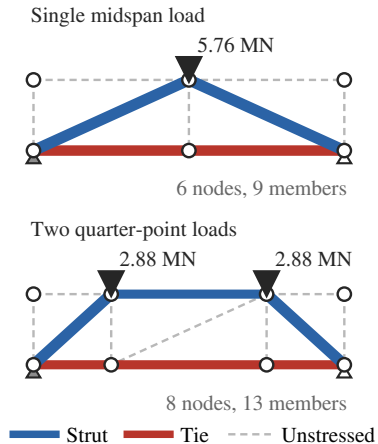
(a) The two loading configurations
