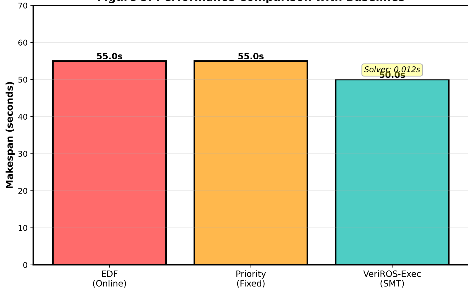
Figure 5: Performance Comparison with Baselines
