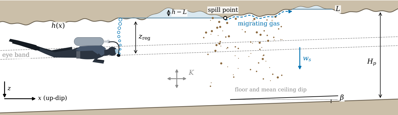
a) Model section along the passage, to scal
