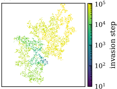
(a) Invasion cluster
