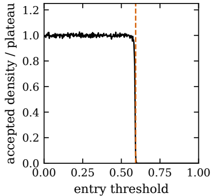
(c) Accepted thresholds
