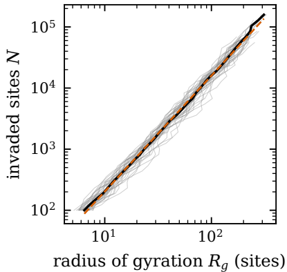
(b) Mass scaling
