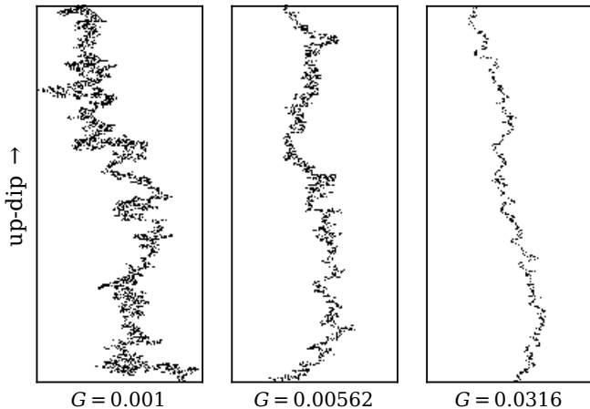
(a) Gas fingers on a dipping smooth ceiling
