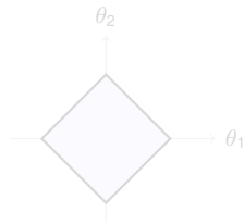
\|\theta\|_1 \leq t : axis-aligned separable, sparse corners
