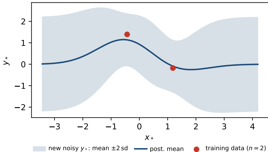
Predictive distribution of a new noisy y_*
