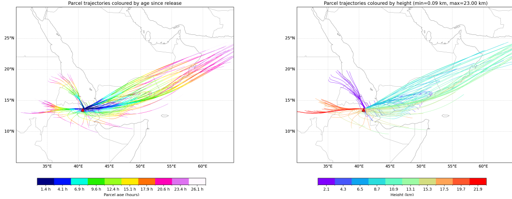
Figure 3: Aggregated forward trajectories for ash ( vash_6 , ..., vash_10 ) colored by age (time since the release) (left) and height (right). Computed by forward in time mode using the Plume-traj tool ( https://github.com/saneku/Plume-traj ).
