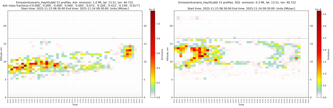
Figure 5: Normalised by erupted mass emission scenarios obtained for ash (left) and \text{SO}_2 (right). Plots are constructed using the PrepEmissSources utility Ukhov and Hoteit [2025]
