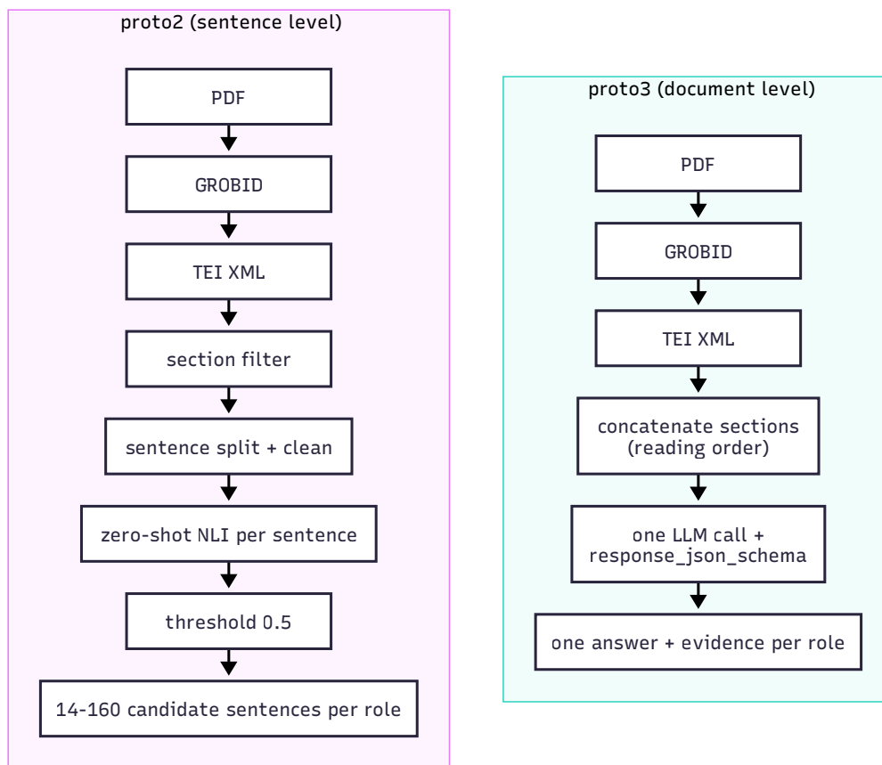
Figure 3: proto2 and proto3 pipelines compared. proto3 removes sentence splitting and the per-sentence acceptance threshold.
