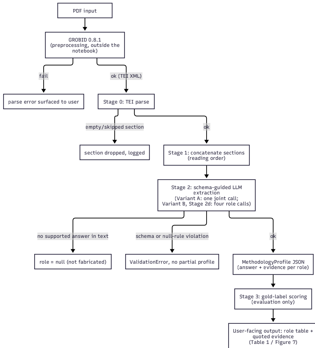
Figure 2: proto3 extraction pipeline with failure paths and the user-facing output step.
