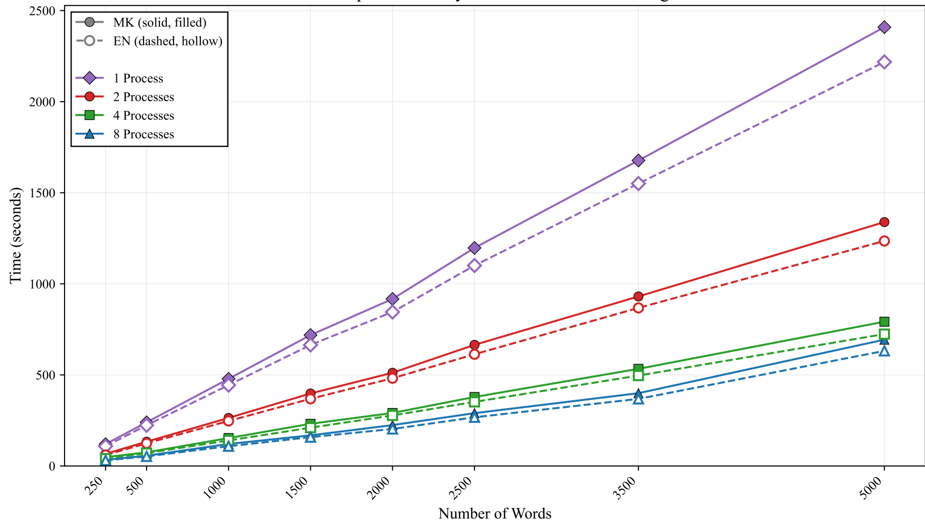
MPI Dict-Split Scalability: Damerau-Levenshtein Algorithm
