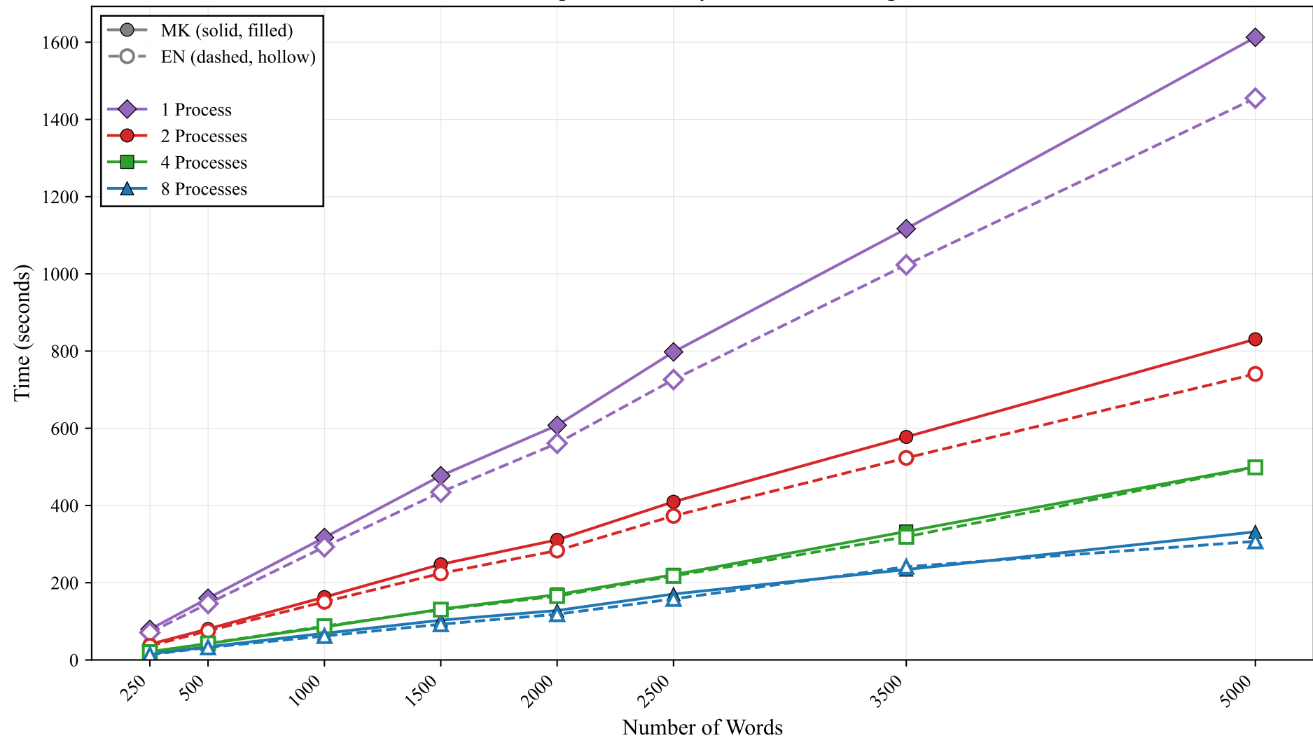
MPI Text-Split Scalability: Levenshtein Algorithm
