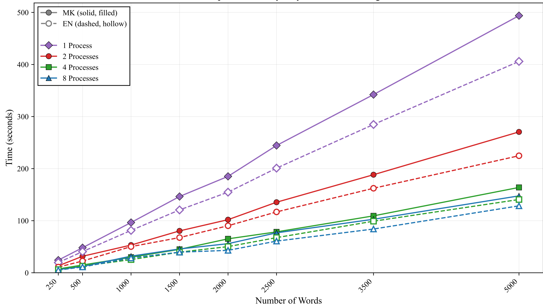
MPI Dict-Split Scalability: Myers Bit-Vector Algorithm
