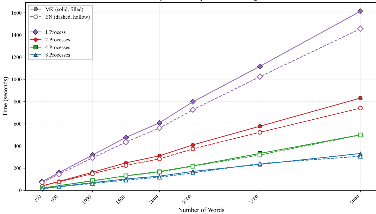
(a) Text-Split: Levenshtein
