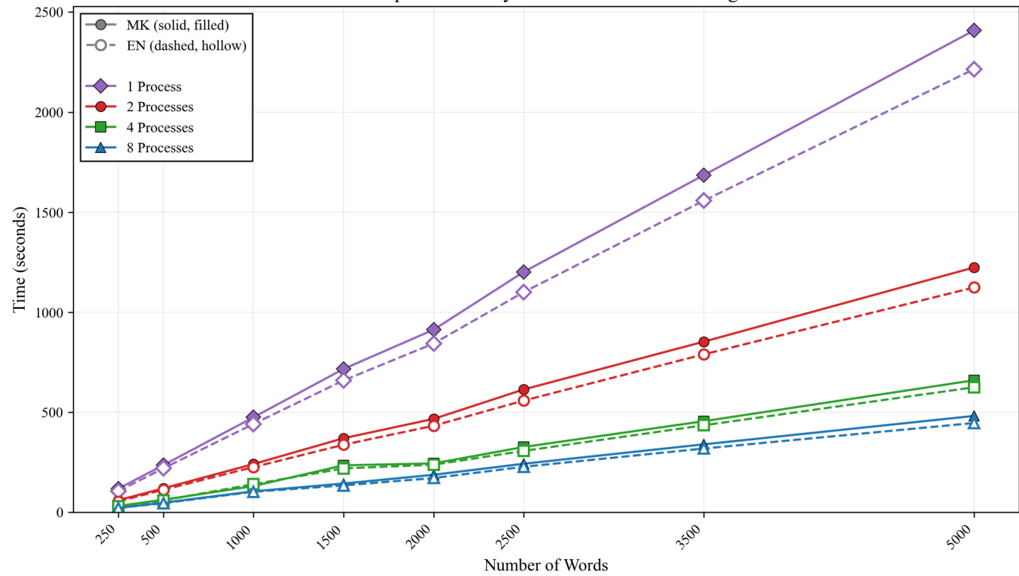
(b) Text-Split: Damerau-Levenshtein
