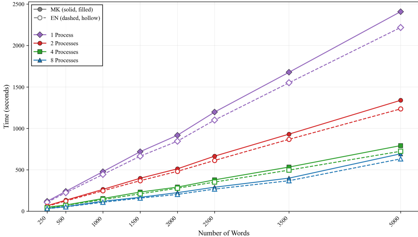
(e) Dict-Split: Damerau-Levenshtein
