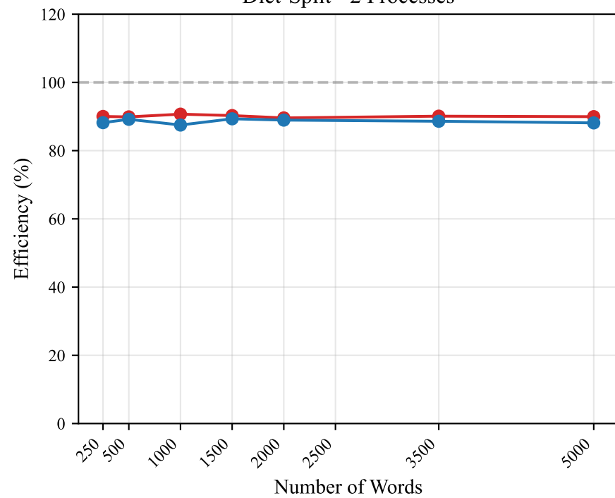
Dict-Split - 2 Processes
