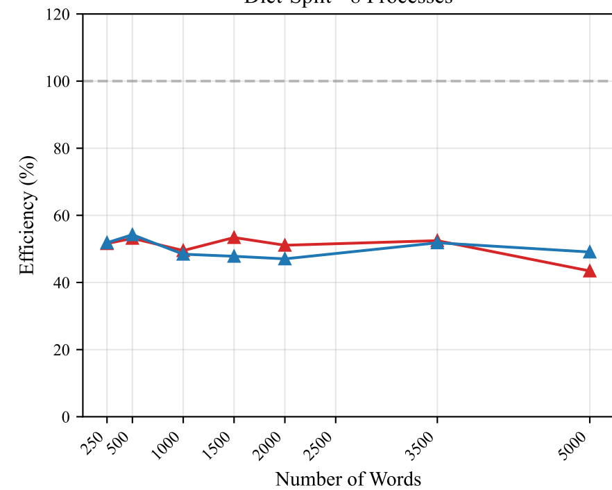
Dict-Split - 8 Processes
