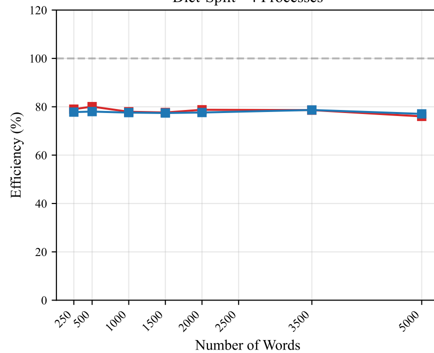
Dict-Split - 4 Processes
