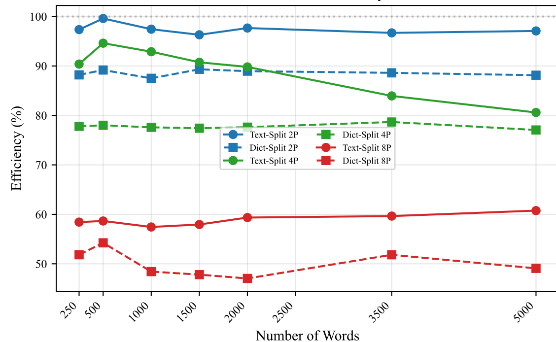
Levenshtein - Efficiency
