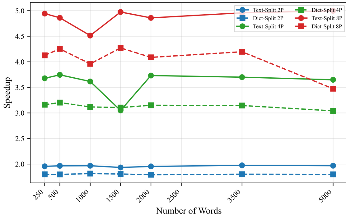
Levenshtein - Speedup
