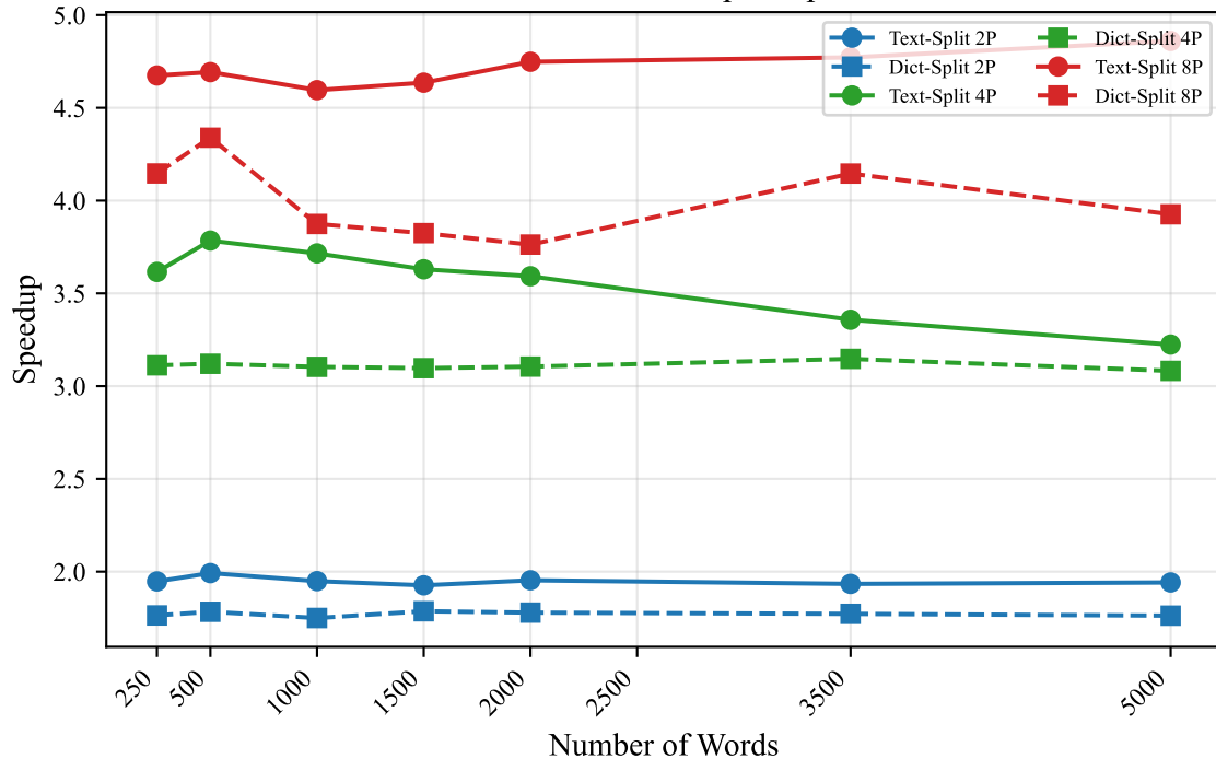
Levenshtein - Speedup
