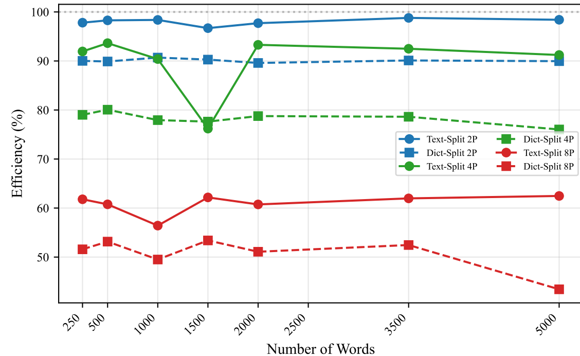
Levenshtein - Efficiency
