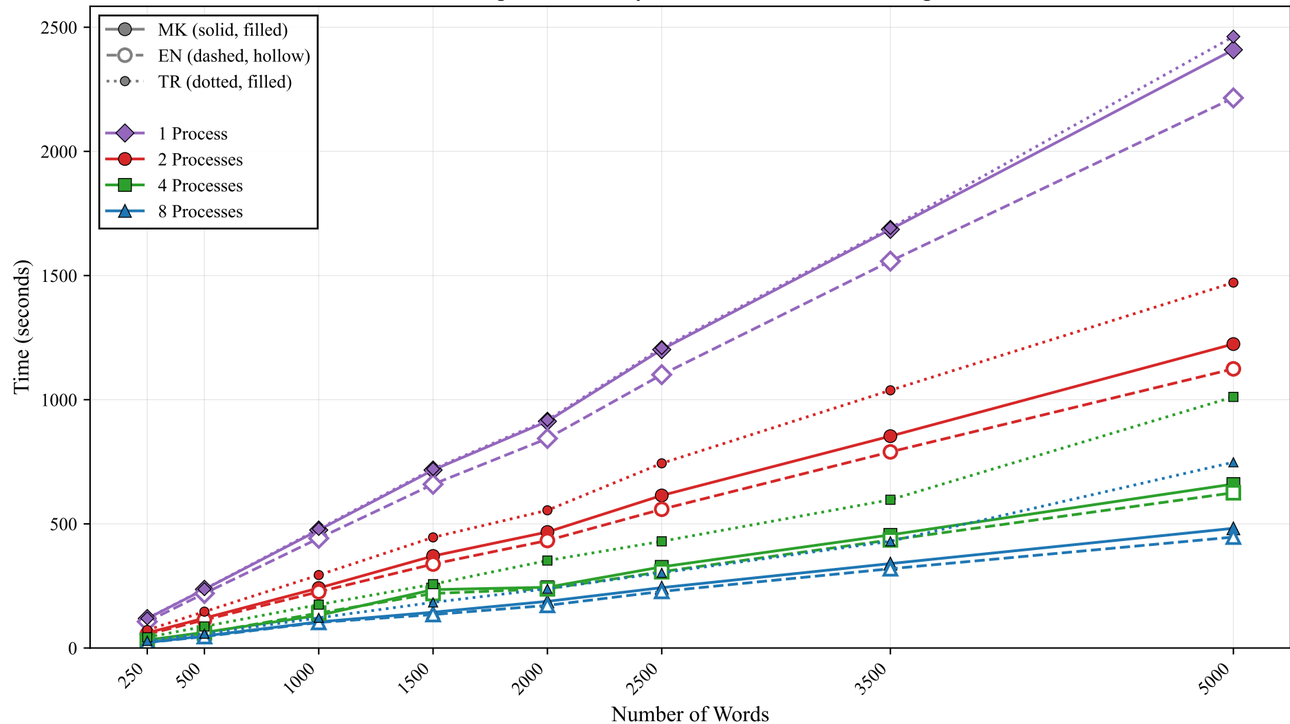
MPI Text-Split Scalability: Damerau-Levenshtein Algorithm
