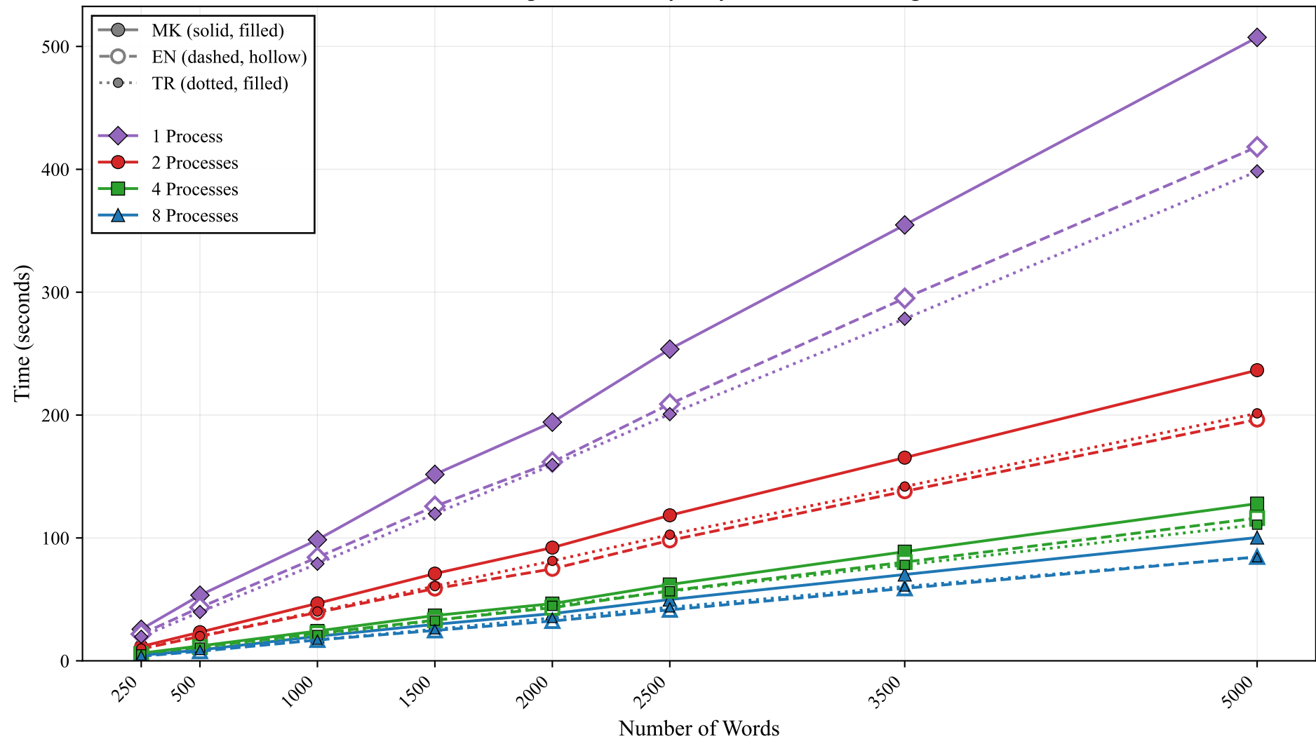
MPI Text-Split Scalability: Myers Bit-Vector Algorithm
