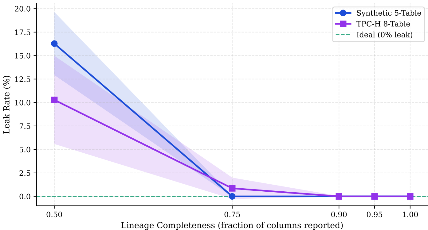
Leak Rate vs. Lineage Completeness (mean \pm std dev, 30 seeds each; completeness=1.0 is honest reporting)
