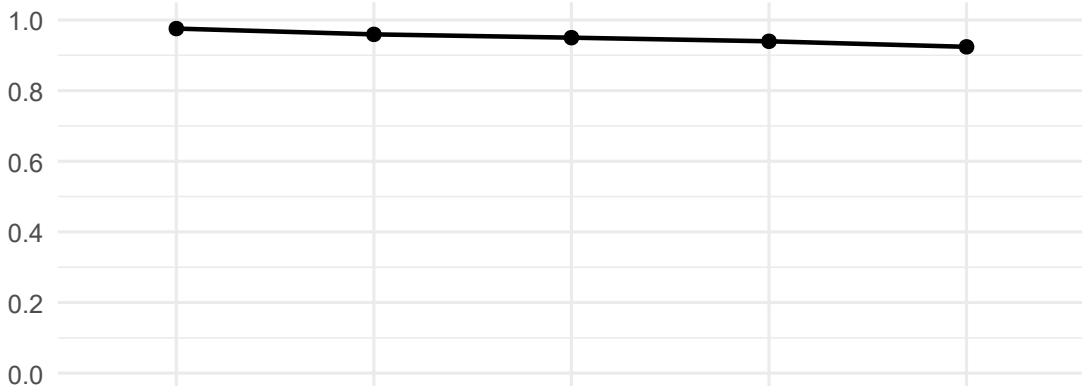
Ridge CCA
