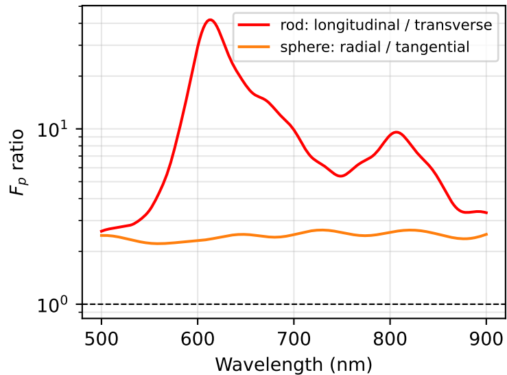
Orientation anisotropy at fixed gap 5 nm
