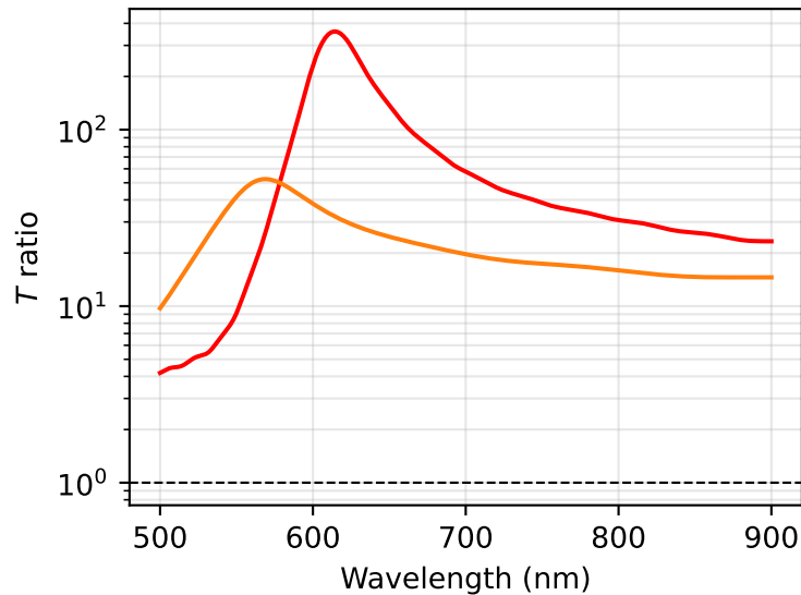
Orientation anisotropy at fixed gap 5 nm
