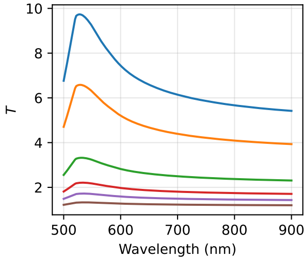
Mie theory: radial dipole near Au sphere R=15.874 nm, gap sweep
