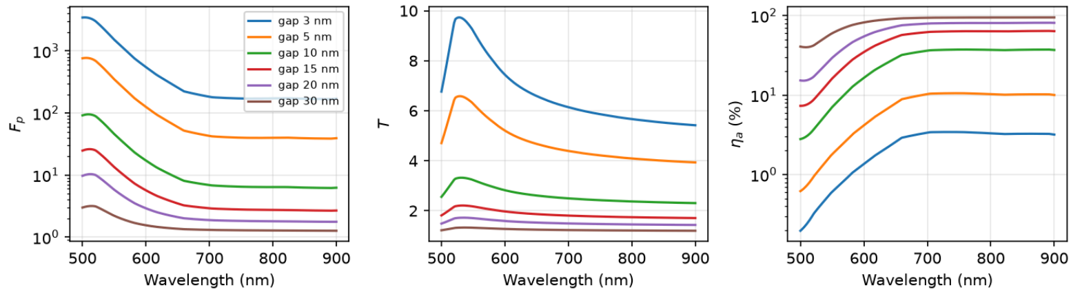
Mie theory: radial dipole near Au sphere R=15.874 nm, gap sweep
