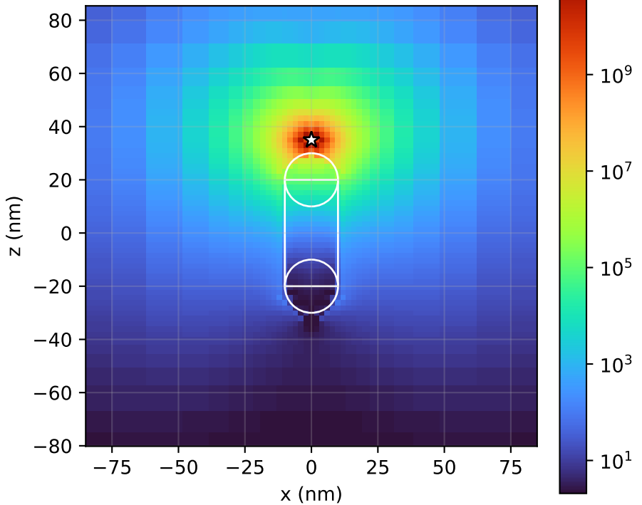
Rod, transverse dipole — 610 nm
