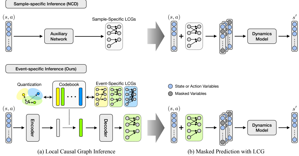
Figure 10. Comparison of the sample-specific inference of NCD ( top ) and quantization-based inference of our method ( bottom ). Event-specific in the diagram refers to inference for a subgroup obtained by quantization.
