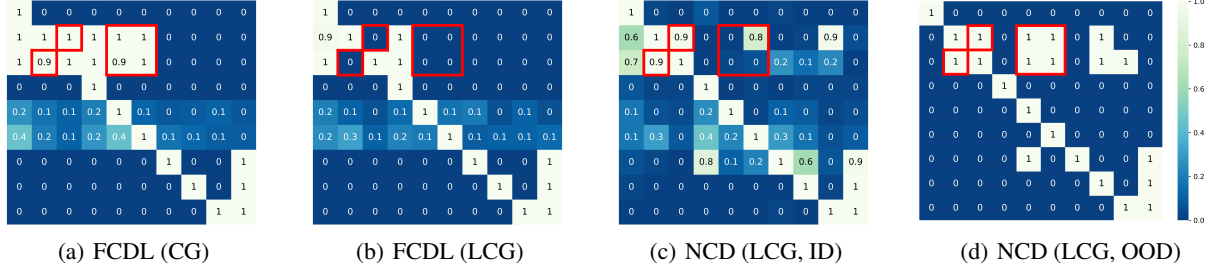
Figure 6. Red boxes indicate edges present in the global reference graph but absent from the non-magnetic reference graph in Fig. 9. (a) CG inferred by our method. (b-d) LCG under the non-magnetic context inferred by (b) our method, and NCD on (c) ID and (d) OOD state.
