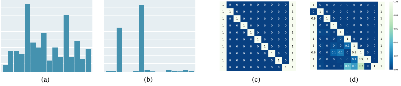
Figure 11. (a,b) Codebook histogram on (a) ID states during training and (b) OOD states during the test in Chemical ( full-fork ). (c) Reference graph for the fork structure. (d) Learned LCG corresponding to the most used code in (b).
