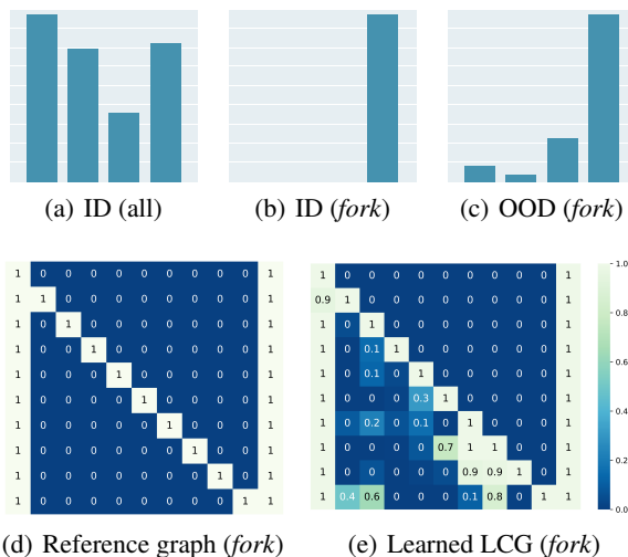
Figure 5. (Top) Codebook histogram of the sample allocations to each of the codes on (a) all ID states, (b) ID states under fork , and (c) OOD states under fork . (Bottom) (d) Reference graph ( fork ). (e) Learned LCG corresponding to the most frequently allocated code in (b) and (c).
