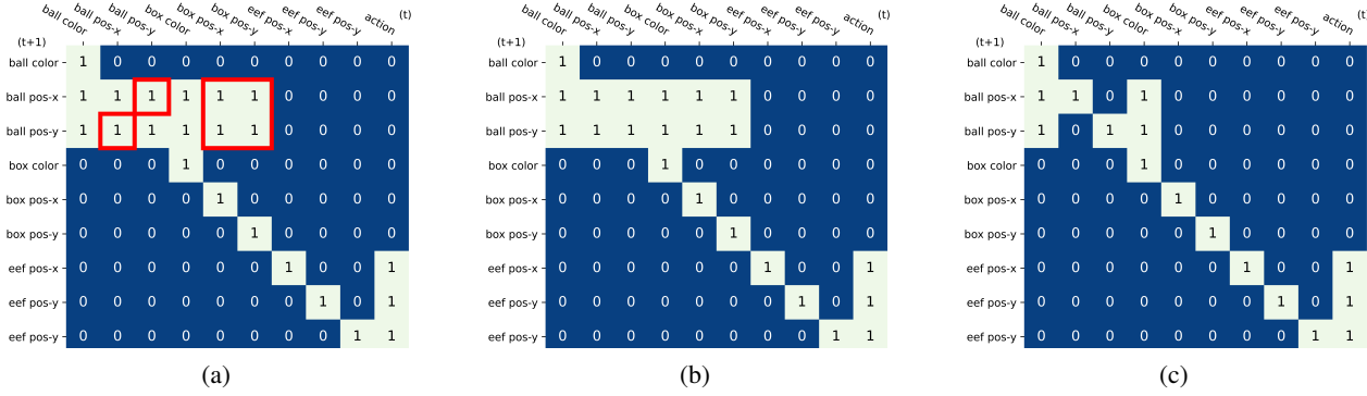
Figure 9. Reference graphs used in the Magnetic experiments: (a) global, (b) magnetic context, and (c) non-magnetic context. Red boxes indicate the six edges by which these references differ; other locally irrelevant edges are retained, as explained in Sec. C.1. The references for the two contexts are not LCGs under Def. 1. The third end-effector coordinate on each axis is z (the repeated eef pos-y label is a typographical error).
