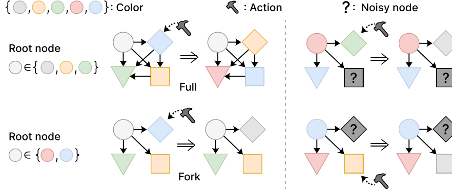
Figure 8. Illustration of CHEMICAL ( full-fork ) environment with 4 nodes. (Left) the color of the root node determines the transition rule. The color partition is schematic: the experiments use red alone for fork , and the other four colors for full . (Right) the noisy nodes are redundant for predicting the colors of other nodes under the fork transition rule.
