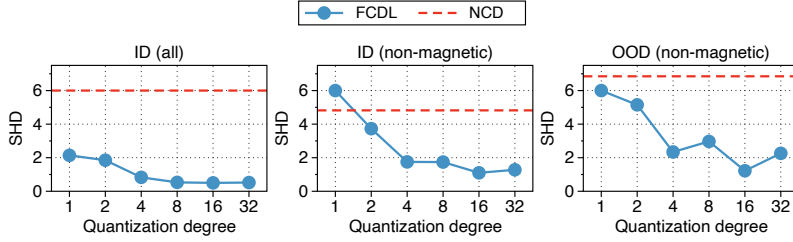
Figure 7. SHD against the reference graphs in Fig. 9 in Magnetic. Recovery of the LCGs defined in Def. 1 has not been re-evaluated.
