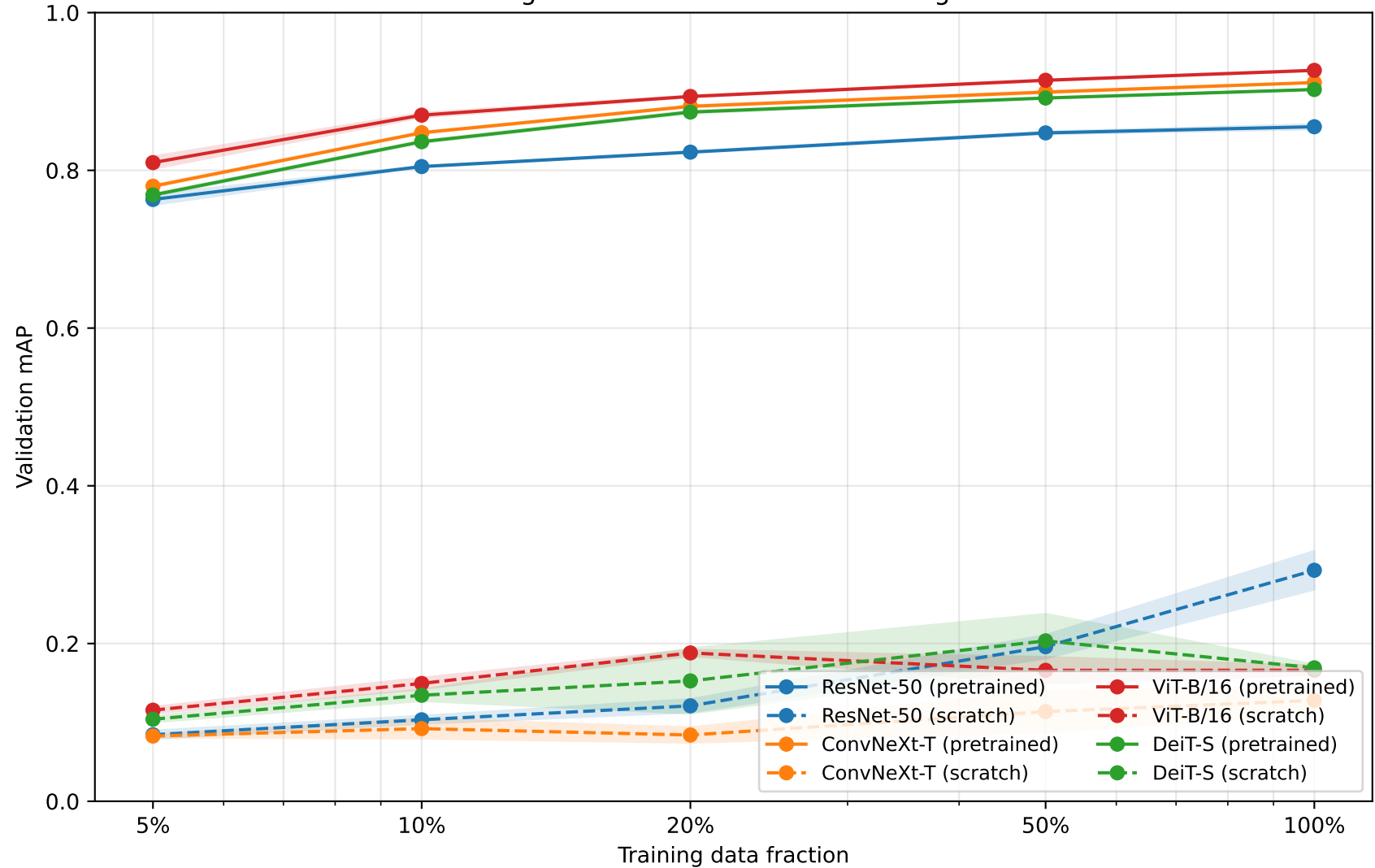
Data-Scaling: 4 Architectures x 2 Pretraining Conditions
