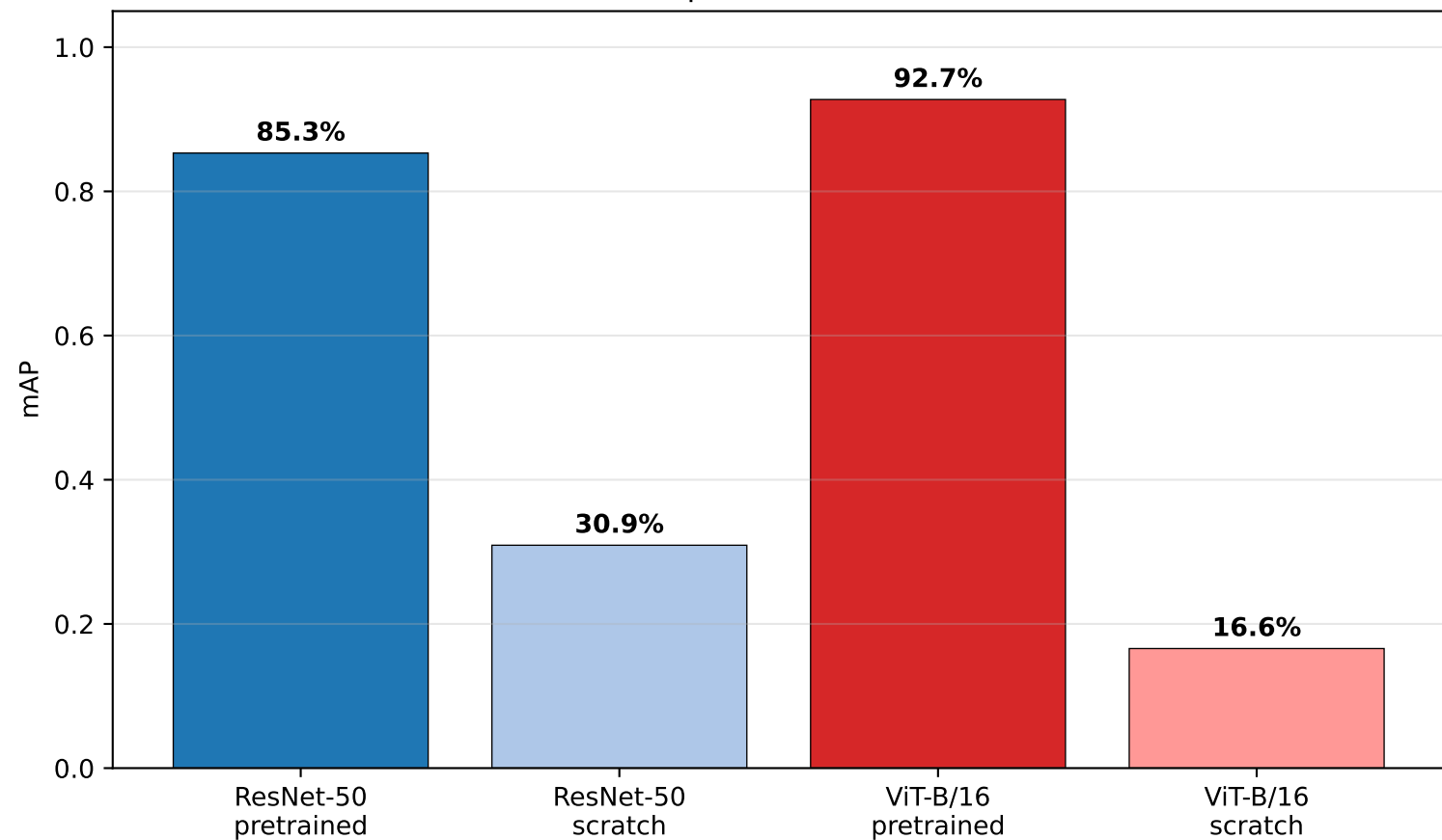
Baseline mAP Comparison (100% data, seed=42)
