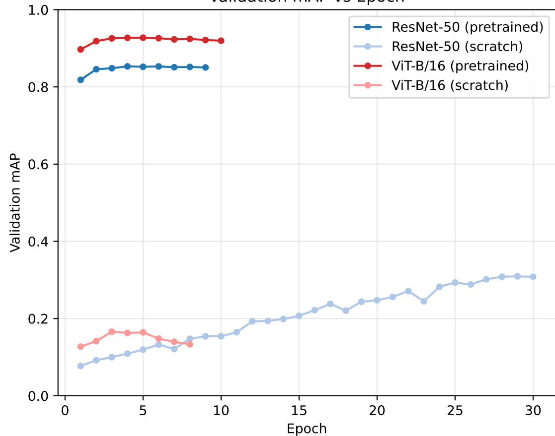
Validation mAP vs Epoch
