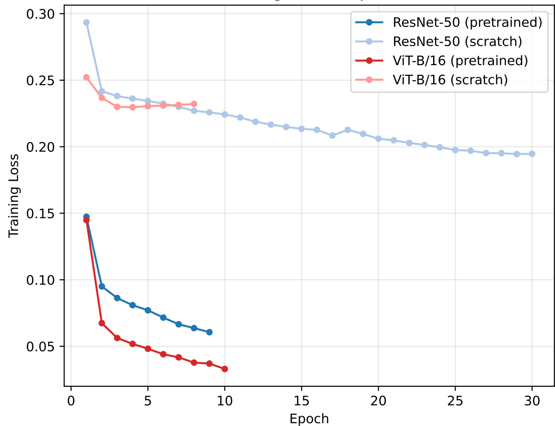
Training Loss vs Epoch
