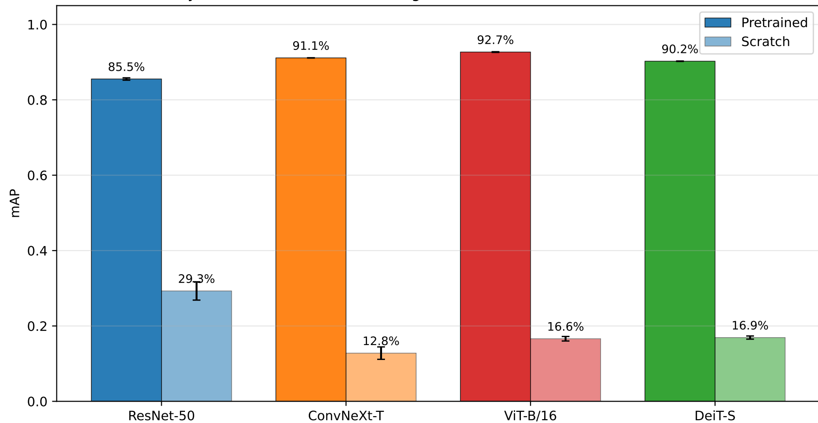
mAP by Architecture and Pretraining (100% data, mean \pm std over 3 seeds)
