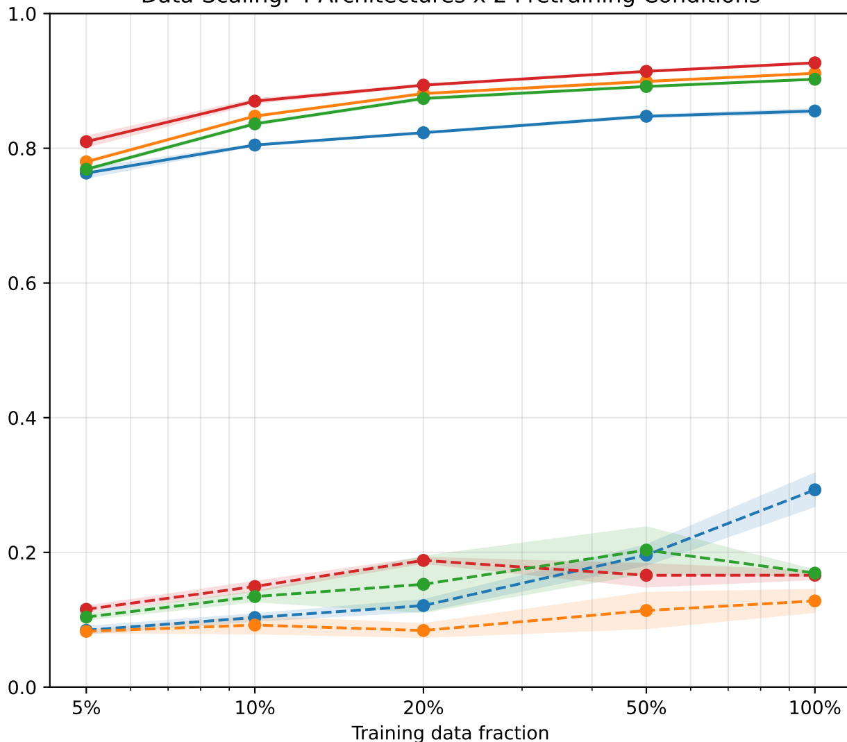
Data-Scaling: 4 Architectures x 2 Pretraining Conditions
