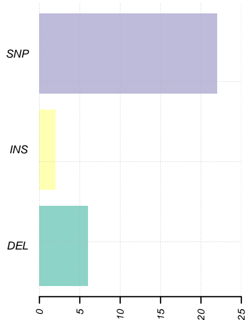
Variant Classification summary
