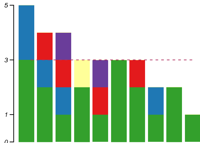
Variants per sample
