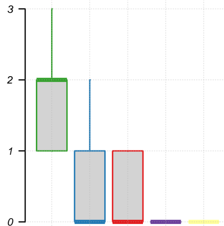
Variant Classification summary
