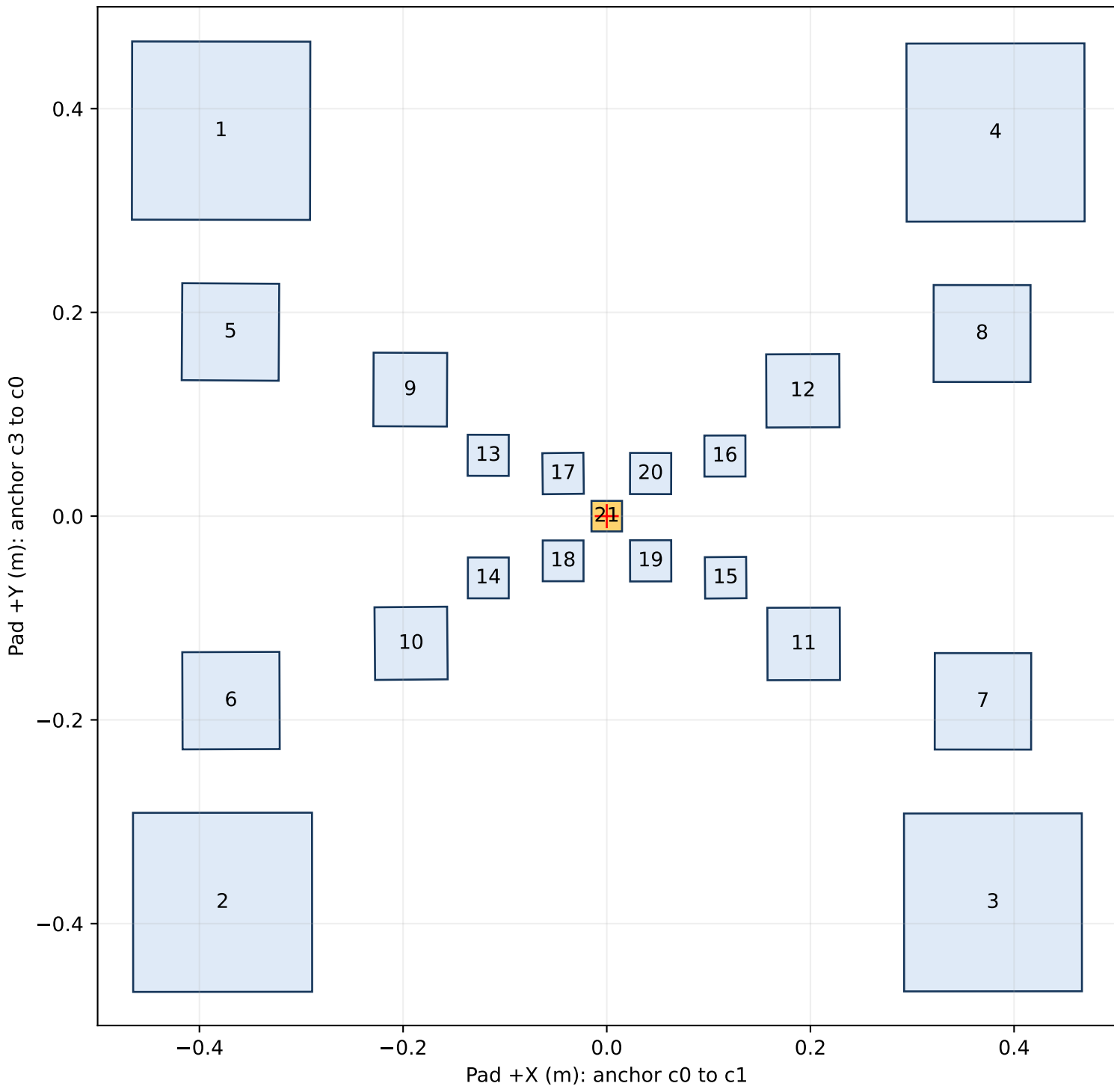
Recovered physical pad — DICT_7X7_50 ID 21 fixed to 30 mm; +Z outward from paper
