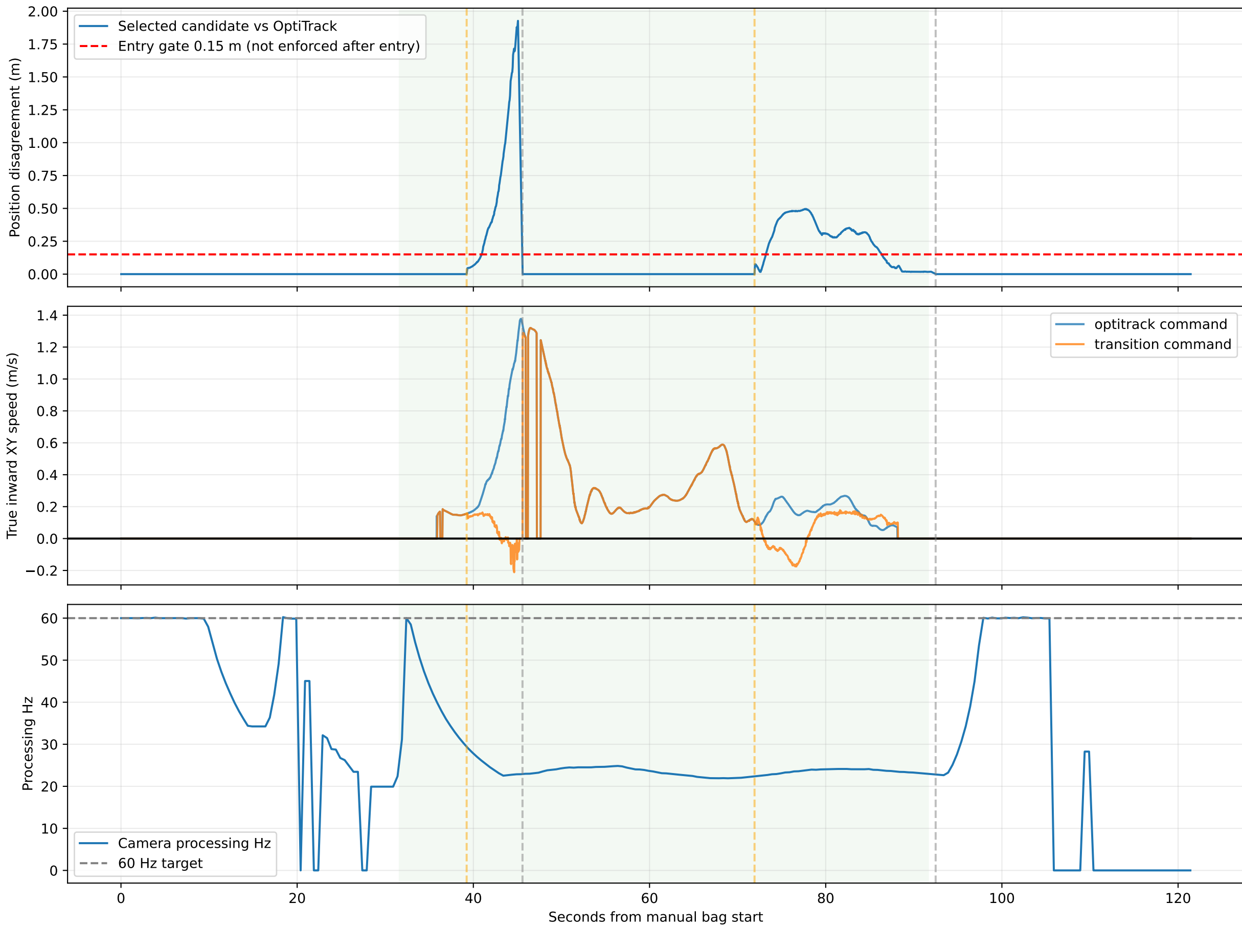
Marker candidate diverges after entry; actual PX4 continued on OptiTrack
