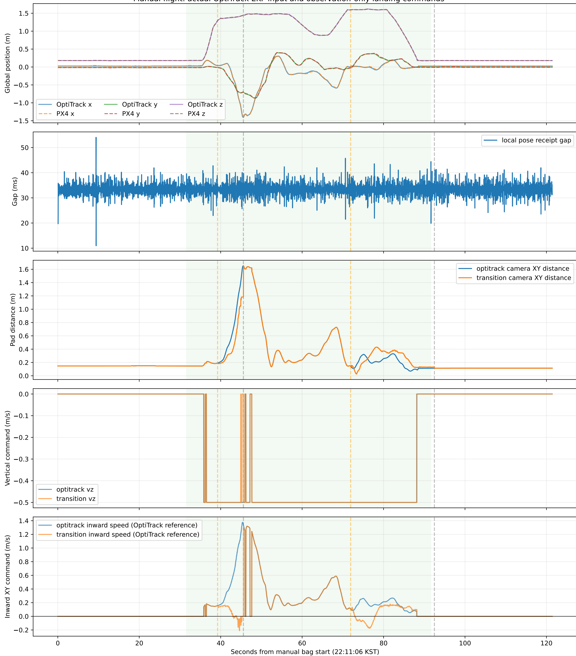
Manual flight: actual OptiTrack EKF input and observation-only landing commands
